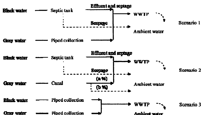
Fig. 2 Scenarios of current and modified wastewater treatment systems in Thailand
