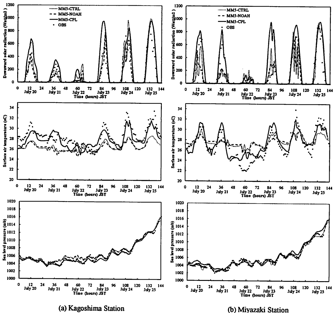
Fig. 5 Downward solar radiation ( \text{Watt/m}^2 ), air temperature at 2m above ground surface ( ^{\circ}\text{C} ) and sea level pressure (mb) at two AMeDAS stations (Kagoshima and Miyazaki) for the different computational cases from 20 to 25 July in 2006.
