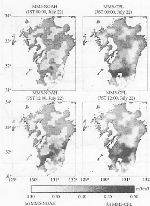
Fig. 6 Soil moisture ( \text{m}^3/\text{m}^3 ) for the different cases on July 22, 2006 every 12hr.
