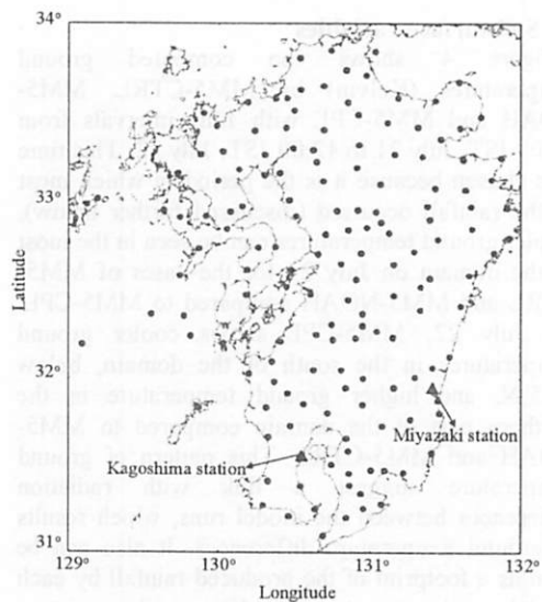
Fig. 3 AMeDAS stations in Kyushu Island (filled circles). Kagoshima and Miyazaki AMeDAS stations are represented by filled triangles.
