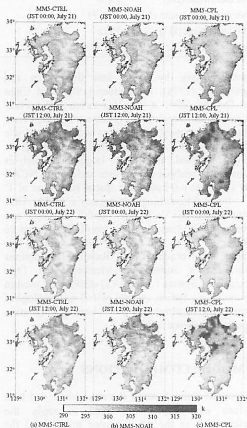
Fig. 4 Ground temperature (Kelvin), for the different cases from 21 to 22 July, 2006 every 12hr.
