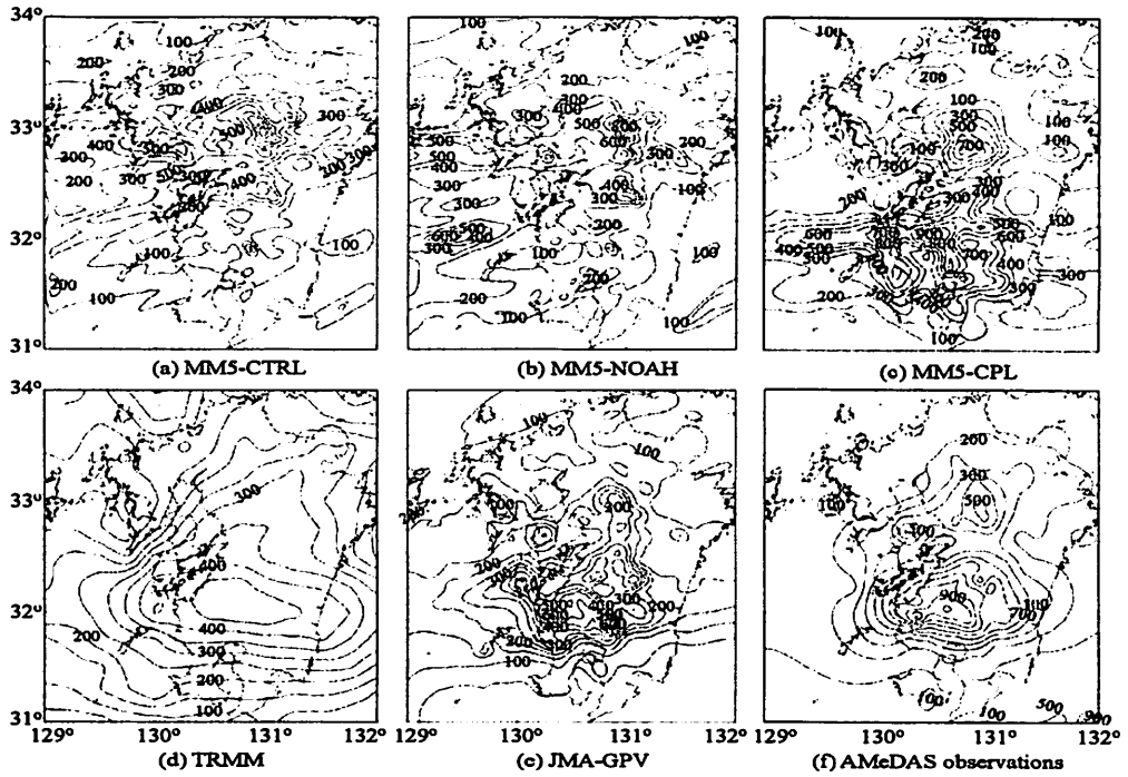
Fig. 8 Isohyets, cumulated in 6 days (from JST 00:00, July 20 to 23:00, July 25, 2006) in mm.
