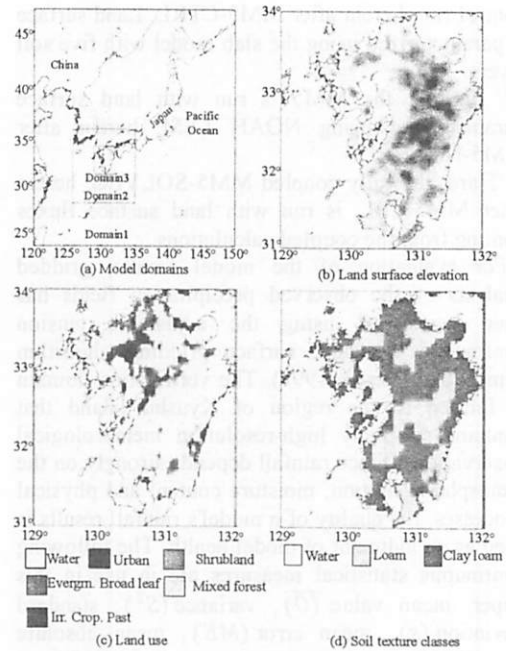
Fig. 2 (a) Domain configurations over Japan, (b) land surface elevation for the third domain (USGS), (c) land use map (USGS) global land use classes, and (d) soil texture classes (FAO+STATSGO).
