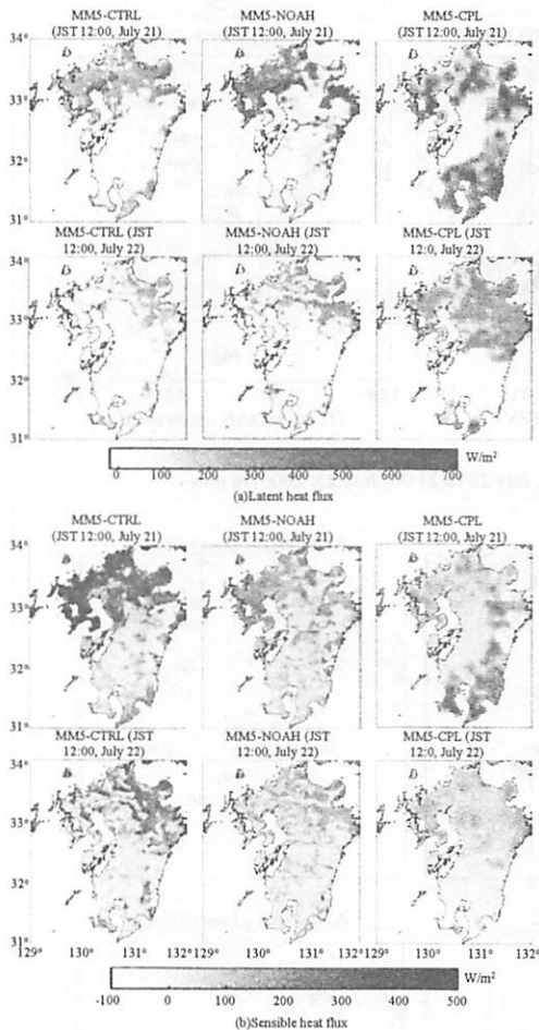
Fig. 7 Latent and sensible heat fluxes ( \text{W/m}^2 ) for the different cases at 12.00 JST, on 21 and 22 July, 2006.
