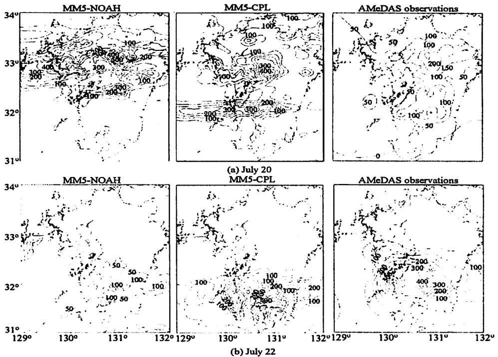
Fig. 9 Total cumulative rainfall (mm) on 20 and 22 July, 2006.
