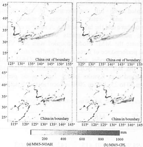
Fig. 10 Total rainfall distribution (from JST 00:00, July 20 to 23:00, July 25, 2006) using different computational domain geometry for the assessment of China land boundary effects on the rainfall simulation.
