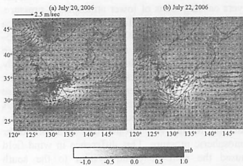
Fig. 11 CPL-NOAH differences of the average daily surface wind vectors, and the average daily sea level pressure over the coarse simulation domain on July 20 and 22.
