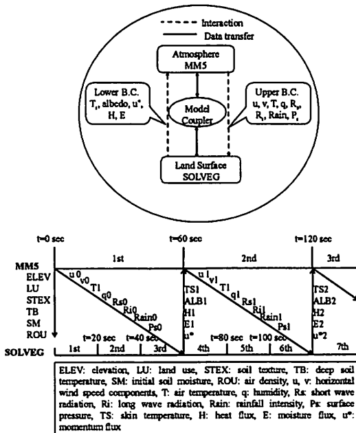
Fig.1 Coupling method and data exchange in the atmosphere land surface coupled model.
