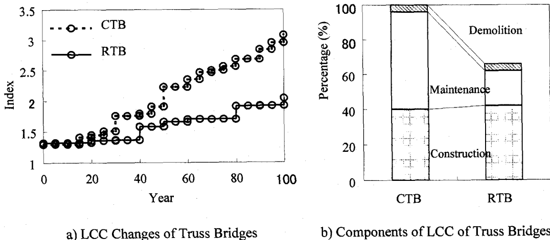
Figure 9. Lifecycle Costs of Truss Bridges
