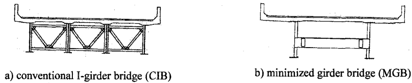
Figure 1. Conceptual Graphs of a Conventional I-girder Bridge and a Minimized Girder Bridge
