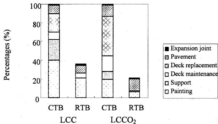
Figure 11. Lifecycle Costs and Environmental Impacts due to Maintenance Activities
