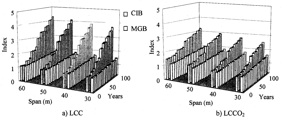
Figure 5. Lifecycle Cost and CO 2 Emission of I-girder Bridges
