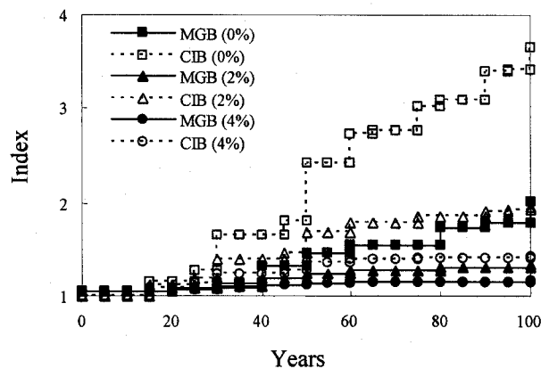
Figure 4. Effects of Discount Rate onto Lifecycle Cost
