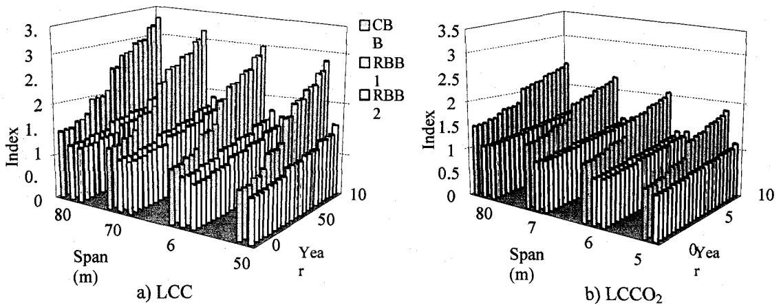
Figure 6. Lifecycle Cost and CO 2 Emission of Box-girder Bridges
