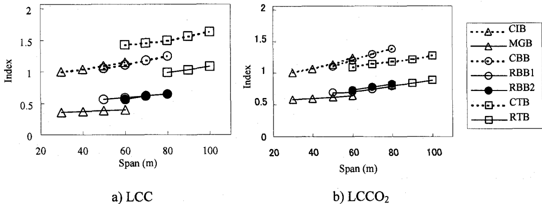
Figure 8. Effects of Bridge Span Lengths in Lifecycle Analysis
