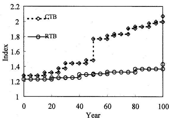
a) LCCO_2 Changes of Truss Bridges
