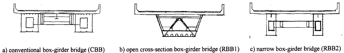
Figure 2. Conceptual Graphs of Conventional and Rationalized Box-girder Bridges
