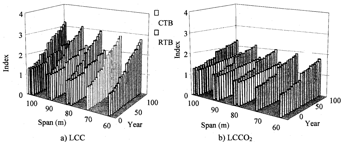
Figure 7. Lifecycle Cost and CO 2 Emission of Truss Bridges
