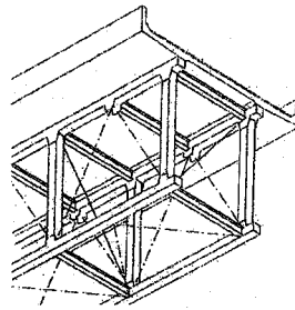
b) rationalized truss bridge (RTB)
