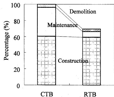
b) Components of LCCO_2 of Truss Bridges
