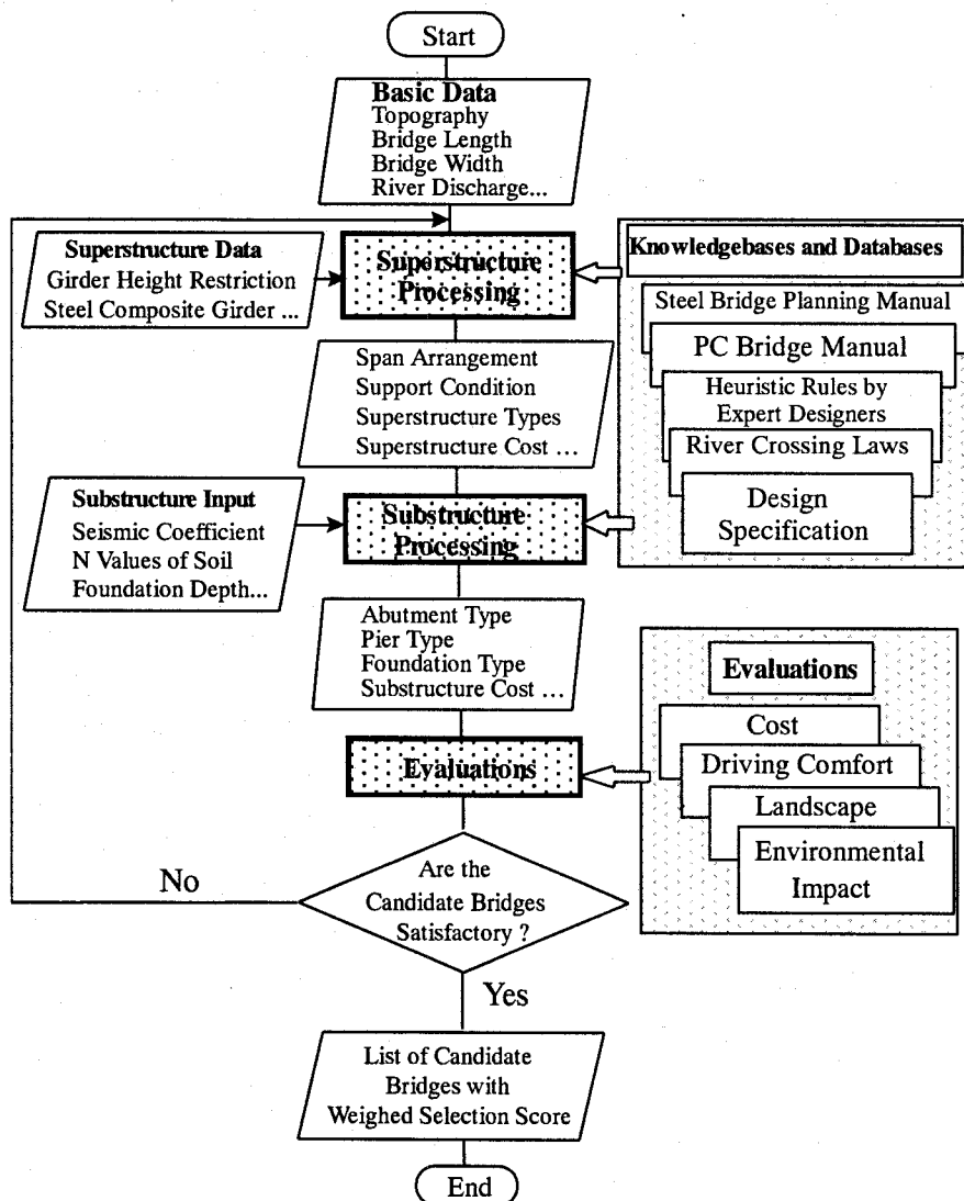
Figure 1. Structure of Bridge Type Selection System
