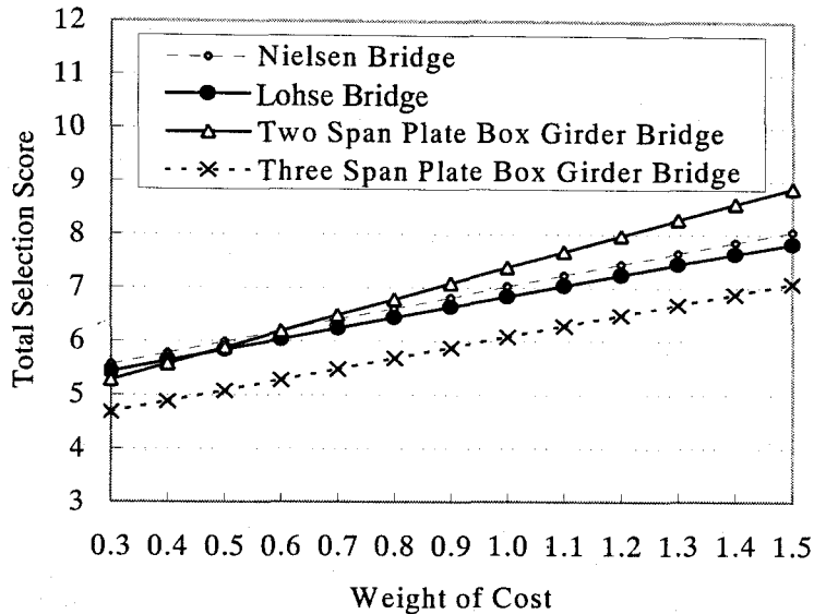
Figure 10. Sensitivity of Total Selection Score with Weight of Cost
