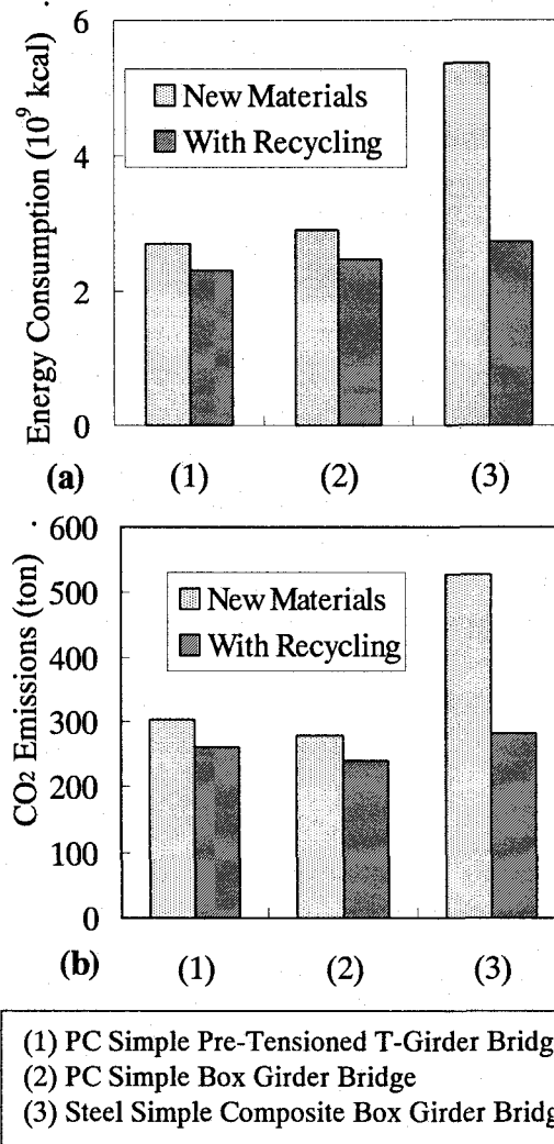
Figure 9. Effect of Recycling on Environmental Impacts (a) Energy Consumption; (b) CO 2 Emissions
