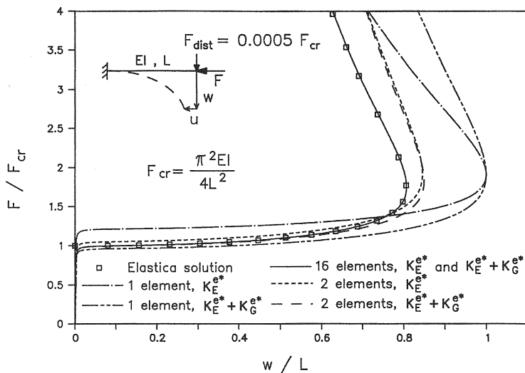
Fig. 4 Load-displacement curves (cantilever beam)
