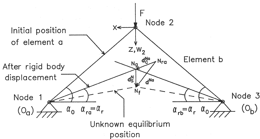
Fig. 2 Two-bar elastic truss
