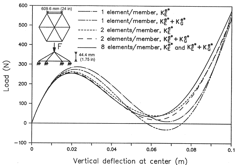
Fig. 6 Load-displacement curves (twelve-member hexagonal frame)
