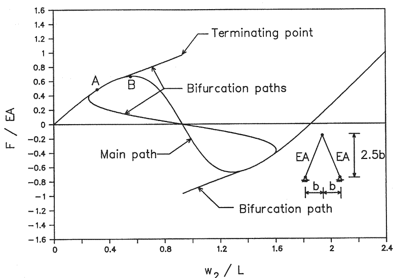
Fig. 3 Load-displacement curves (two-bar truss)
