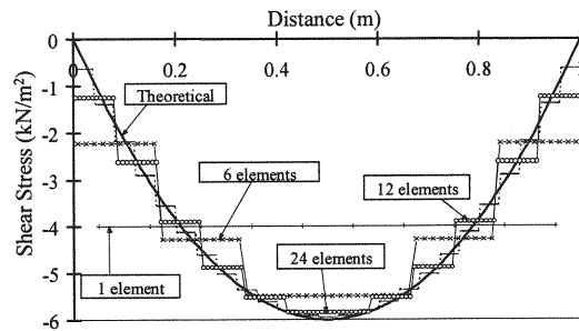
Fig. 8 Shear stress distribution at section A-A
