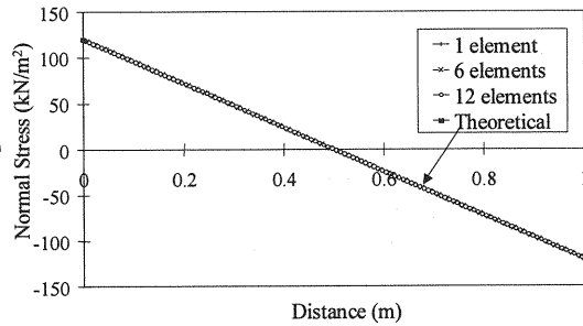
Fig. 7 Normal stress distribution at section A-A
