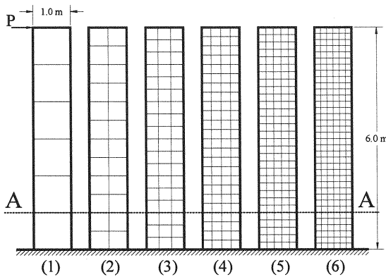
Fig. 5 Dimensions and element arrangements of laterally loaded cantilever models
