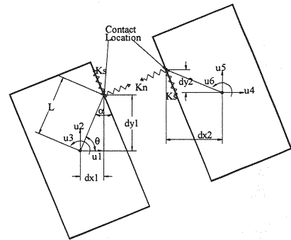
Fig. 2 Element shape, contact location and degrees of freedom
