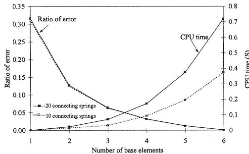
Fig. 6 Relations between the number of base elements, ratio of error and CPU time
