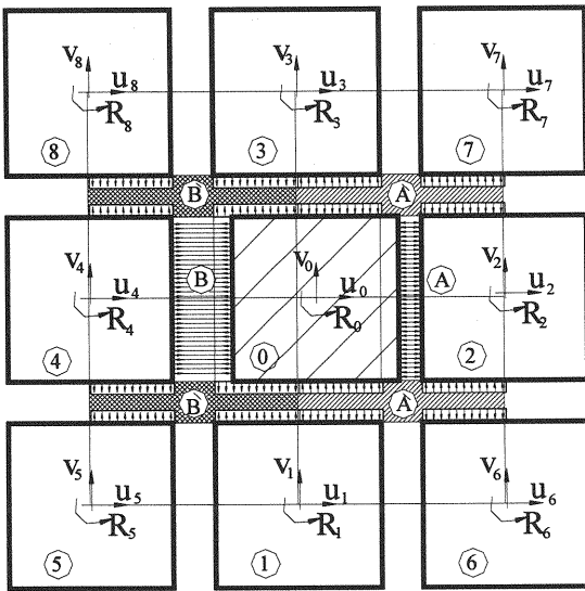
Fig. 11 Secondary stresses due to horizontal displacement of the element (0)
