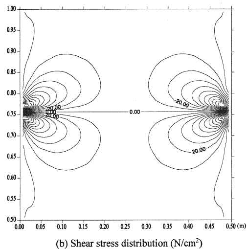
Fig. 19 Stress contour around the reinforcement bar location
