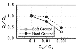
(e) Reduction Ratio of Shear Forces of Center Wall
