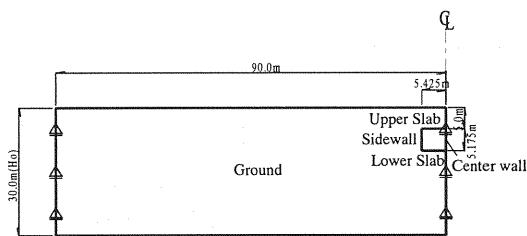
Fig.2 Model for 2D FE Analysis
