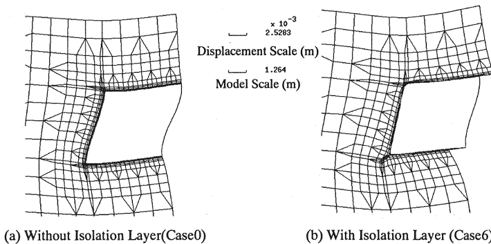
Fig.6 Displacement around Tunnel for Shear Force
