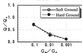
(b) Reduction Ratio of Shear Forces of Sidewall
