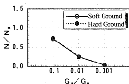
(c) Reduction Ratio of Axial Force of Sidewall
