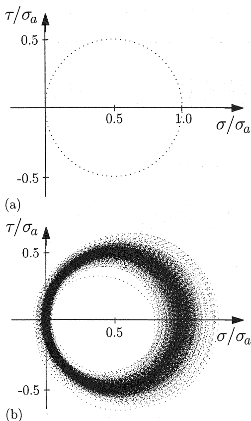
Fig. 6 (\sigma_\theta, \tau_\theta) traces for network nodes defined at: a) cell nucleus; and b) cell area centroid
