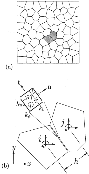
Fig. 1 Rigid-Body-Spring Model: a) partitioning of domain using a Voronoi diagram; b) elemental unit
