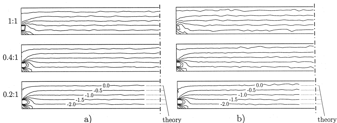
Fig. 9 Contours of \sigma_x/\sigma_F provided by: a) RBS network; b) CST finite elements
