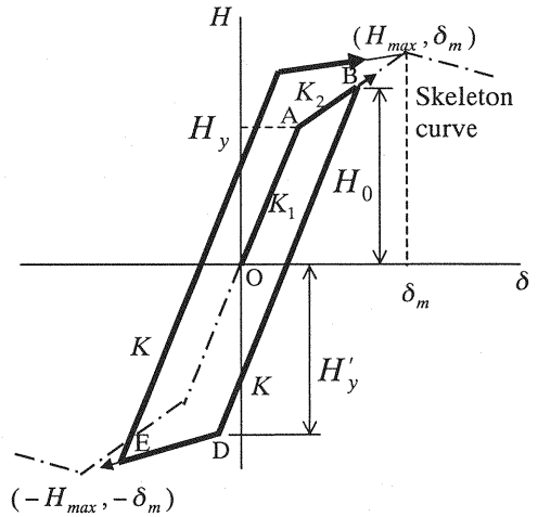
Fig.6 Hysteretic rules of the hardening stage (2-para model)
