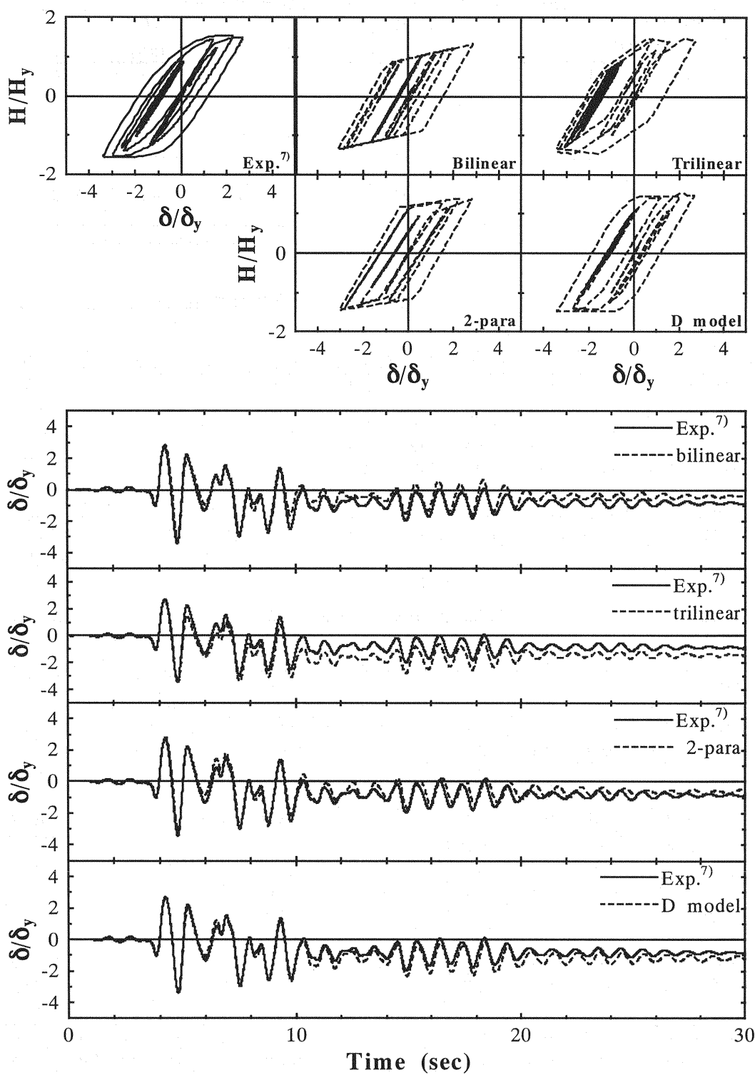
Fig.9 Simulation of Pseudodynamic test (TS08-30-18(JMA))
