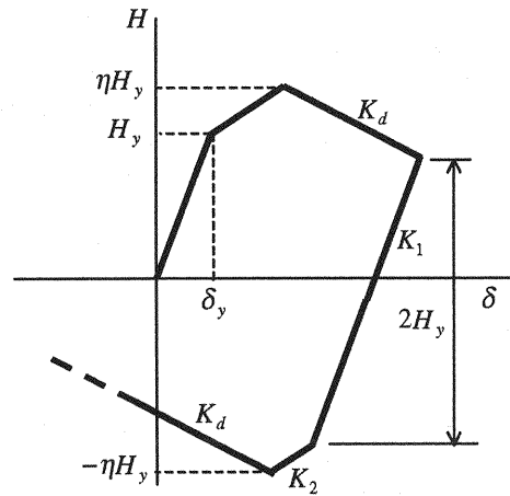
Fig.3 Hysteretic rules of trilinear model
