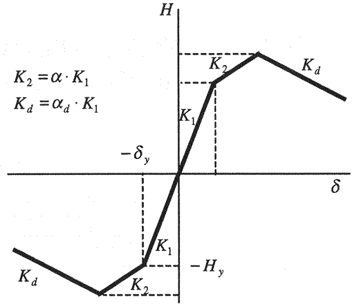
Fig.2 Primary curve of trilinear model
