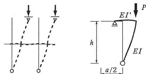
(b) hinged support
