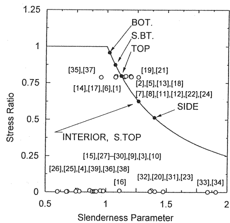
Fig. 10 Stability state of units in Example ( 2 )
