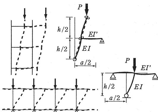
Fig. 3 Units of side column and top column
