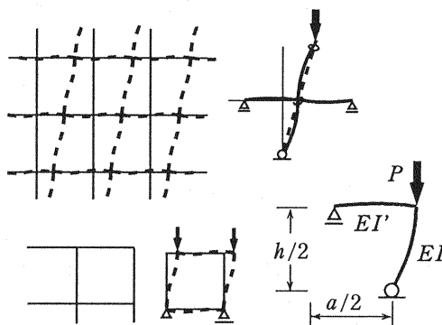
Fig. 2 Unit of interior column
