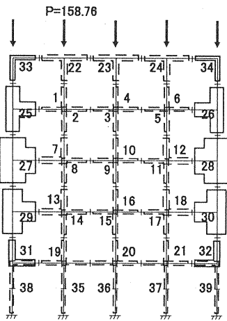
Fig. 7 Quadratic work of units in Example ( 1 )
