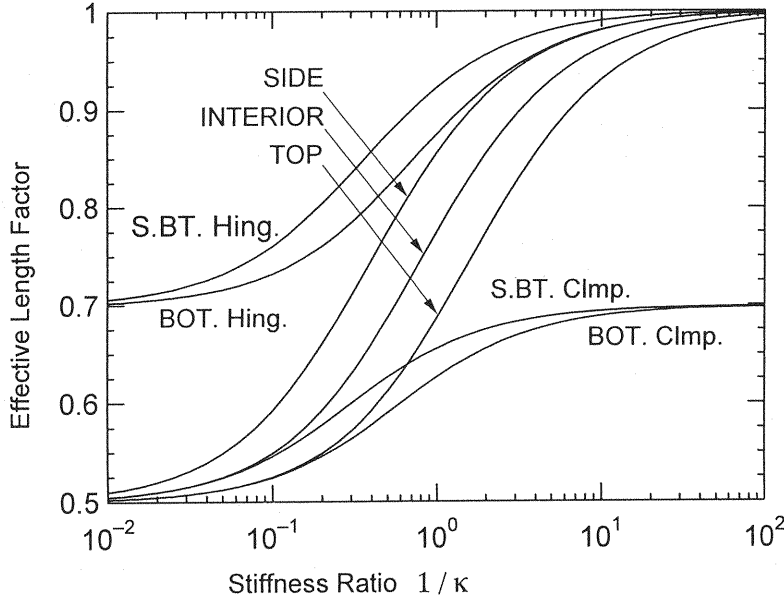
Fig. 14 Effective length factor of column units / braced
