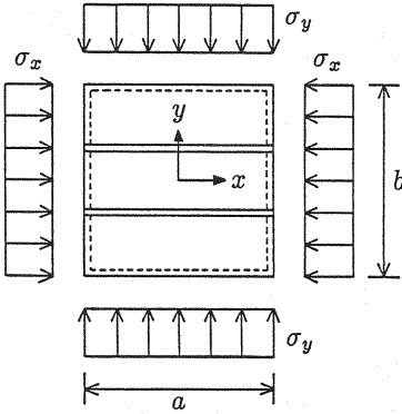
Fig. 1-a Biaxially forced stiffened plates.
