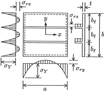
Fig. 1-b Residual stress distributions.
