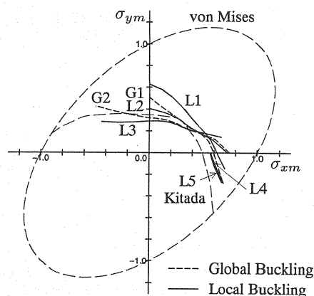
Fig. 9 Interaction curves for square stiffened plates ( b_e/t = 60, W_o t = b_e/150 ).
