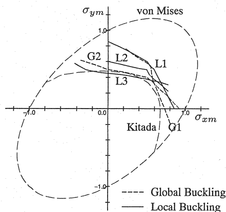
Fig. 8 Interaction curves for square stiffened plates ( b_e/t = 40, W_o t = b_e/150 ).
