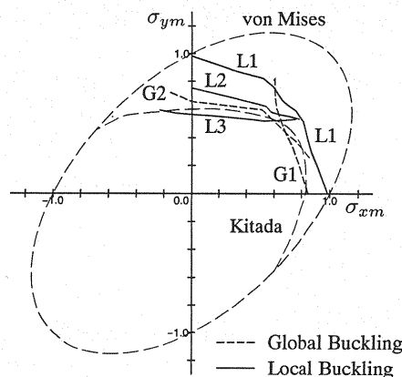
Fig. 7 Interaction curves for square stiffened plates ( b_e/t = 30, W_o t = b_e/150 ).
