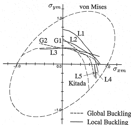
Fig. 6 Interaction curves for square stiffened plates ( b_e/t = 60, W_o t = a/1000 ).
