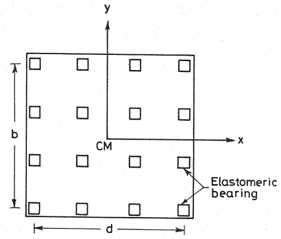
Fig.2 Arrangement of the bearings
