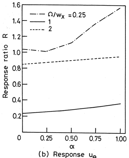
Fig.11 Variation of ratio R for u_y and u_\theta against \alpha . T_x=1 sec., e_x/d=0.25 , m_b/m=2 , Q=50 ton and w_\theta/w_x=1 .
