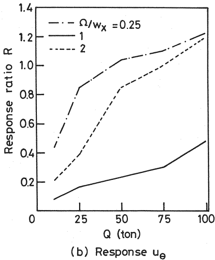
Fig.10 Variation of ratio R for u_y and u_\theta against Q . T_x=1 sec., e_x/d=0.25 , m_b/m=2 , w_\theta/w_x=1 and \alpha=0 .
