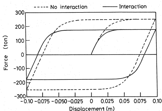
Fig.3 Force deformation characteristic of the bearing.
