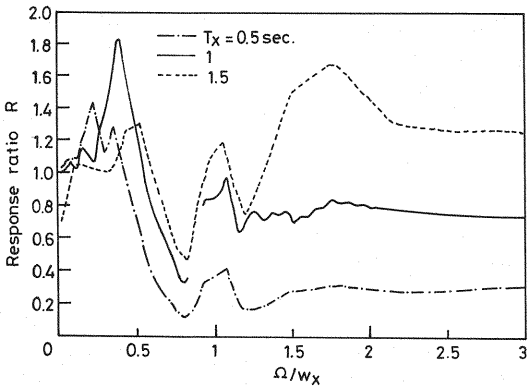
Fig.5 Variation of response ratio R for response u_y . e_x/d=0.25 , m_b/m=2 , w_\theta/w_x=1 , Q=50 ton and \alpha=0 .
