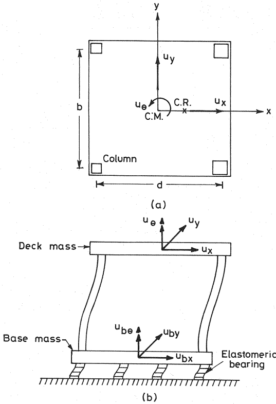
Fig.1 Structural model
