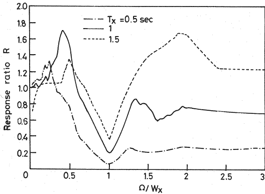
Fig.4 Variation of response ratio R for response u_x . e_x/d=0.25 , m_b/m=2 , w_\theta/w_x=1 , Q=50 ton and \alpha=0 .
