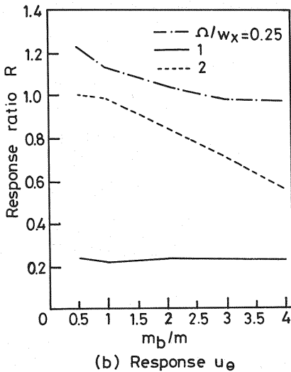
Fig.8 Variation of ratio R for u_y and u_\theta against m_b/m . T_x=1 sec., e_x/d=0.25 , w_\theta/w_x=1 , Q=50 ton and \alpha=0 .
