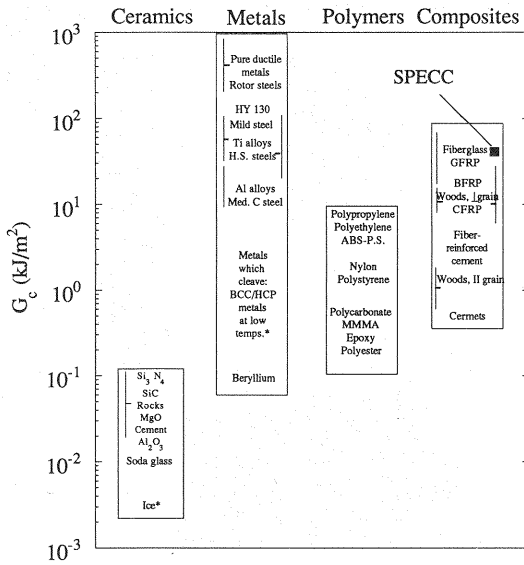
Fig.13 Comparison of Fracture Energy of Spectra ECC with other Structural Materials (adapted from Ashby and Jones, 1984).
