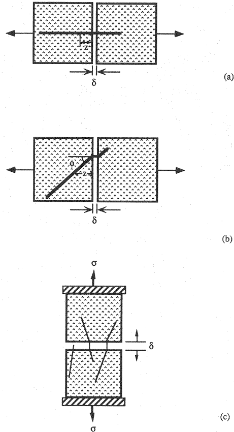
Fig.5 Three Essential Steps in Deriving the \sigma-\delta Relation for Short Random Fiber Reinforced Cementitious Composites (a) Single Fiber Normal Pull-Out. The fiber bridging stress is \sigma_s(\delta, z) ; (b) Inclined Fiber Pull-Out. The fiber bridging stress is \sigma_s(\delta, z, \phi) ; (c) Statistical Description of Fiber Distribution.
