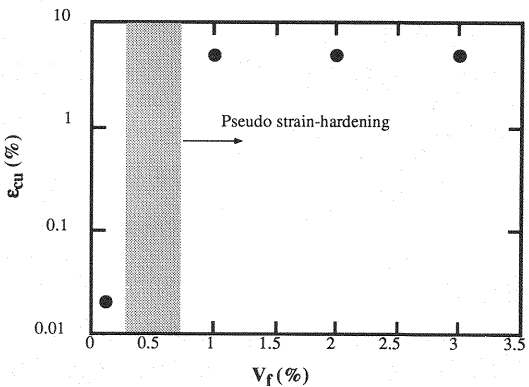
Fig.6 Strain Capacity of Spectra ECC for Various Fiber Volume Fractions. The estimated critical fiber volume fraction is indicated by the shaded strip.
