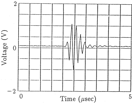
Fig.4 Measured ultrasonic pulse.
