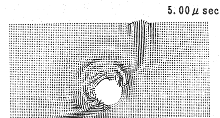
(c) Angled wave method ; circular hole
