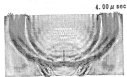
(b) Normal wave method ; slit
