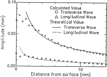
Fig.9 Damping properties of simulated waves.
