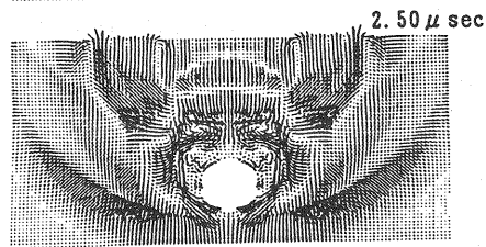
(a) Normal wave method ; circular hole
