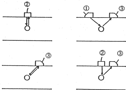
Fig.2 Location of Probes.
