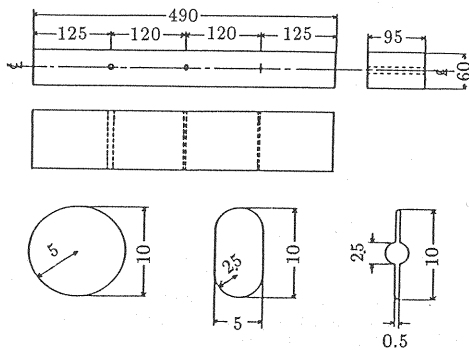
Fig.1 Steel test specimen
