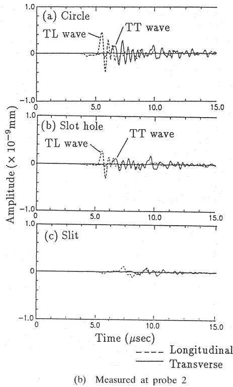
(b) Measured at probe 2
