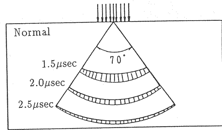
Fig.7 Simulation of normal wave.
