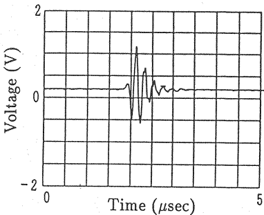
(a) Circular hole
