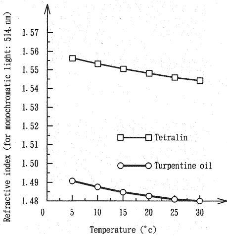
Fig.3 Variation of refractive index of solvents with temperature.
