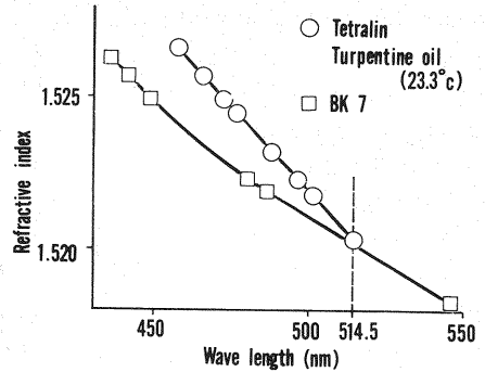
Fig.5 Variation of refractive index with wave length.
