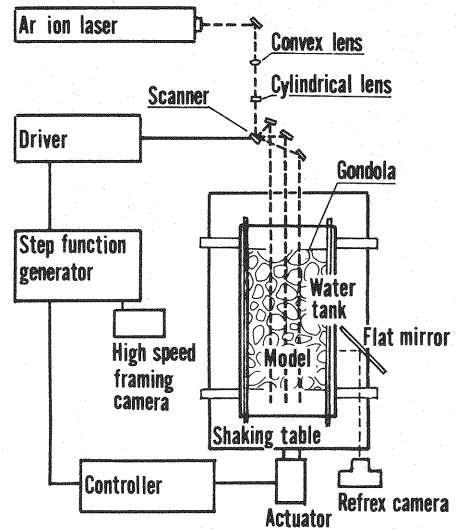
Fig.13 Apparatus for dynamic failure test.
