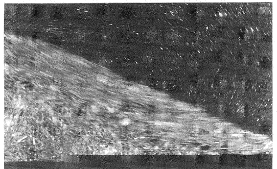
Fig.14,b Excitement frequency = 22 Hz, base acceleration = 153.4 – 162.3 gal.
