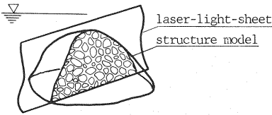
Fig.1 Visualization method.
