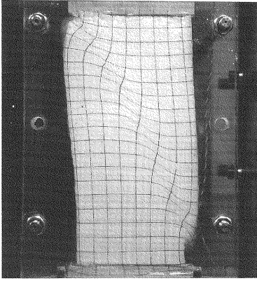
Fig.12 Failure pattern of the glass particles in PSC test, at \epsilon_a = 12\% , \sigma_c = 0.05 \text{ kgf/cm}^2 and e = 0.840 .
