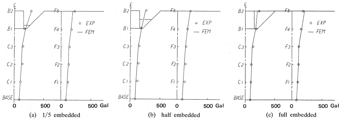
Fig.12 The maximum acceleration distribution from the experimental and simulated results under the same input motion; 80Gal
