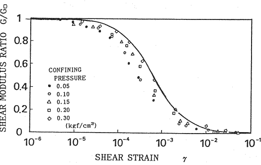
Fig.7 The strain dependency of the shear modulus ratio
