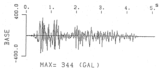
Fig.9 An acceleration time trace of the scaled input motion
