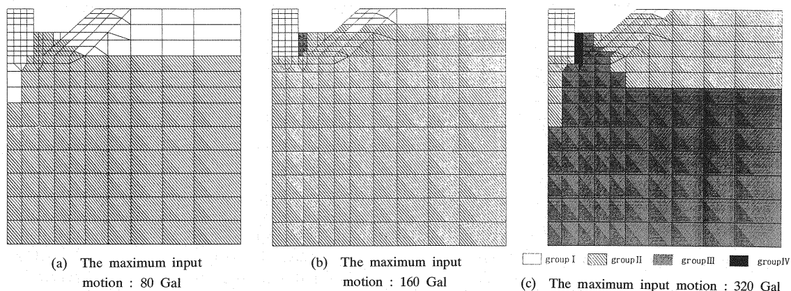
Fig.16 The maximum shear strain distribution induced in the soil; Half embedment( d=15\text{cm} )
