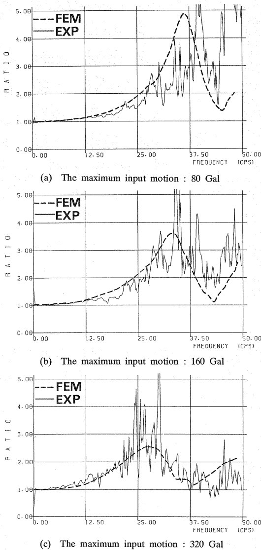
Fig.15 The transfer functions (B2/F4) obtained from the experiment and the simulation
