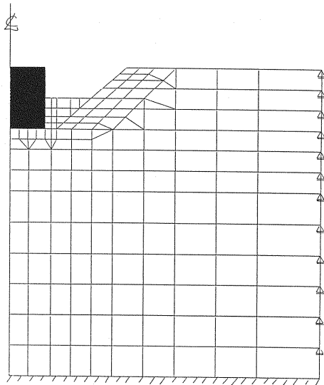
Fig.11 An axi-symmetric finite element model of the soil-foundation system
