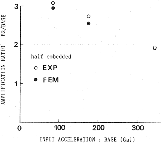
Fig.14 The maximum amplification ratio (B2/BASE) versus the maximum BASE acceleration
