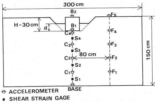
Fig.2 The vertical cross section of the model ground-foundation system
