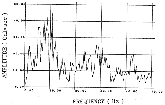
Fig.10 Fourie spectrum of the scaled input motion
