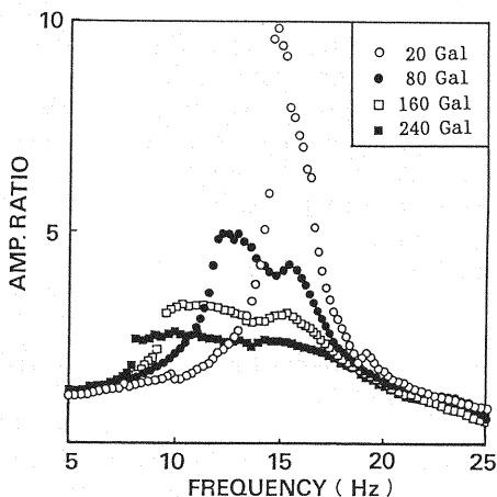
Fig.3 The resonance curves of the ground obtained from steady state response
