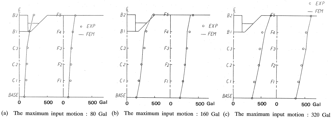
Fig.13 The maximum acceleration distribution of from the experimental and simulated results under the same embedment depth ; half embedded
