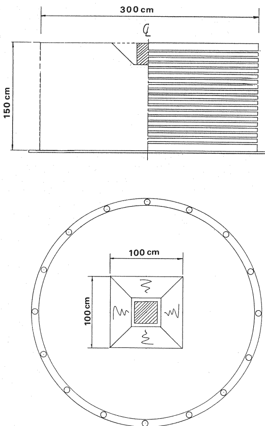
Fig.1 A cylindrical large soil container on the shaking table
