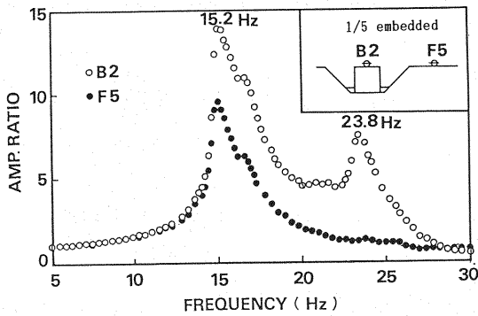
Fig.5 The resonance curves of the soil-foundation system subjected to 20Gal input motion
