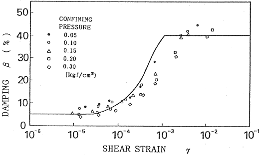
Fig.8 The strain dependency of the damping
