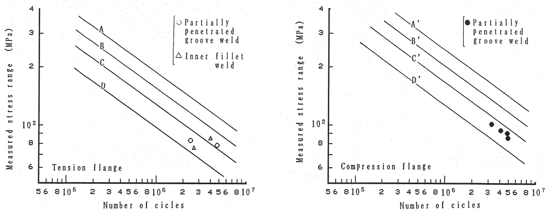
Fig.8 Fatigue Test Results (Measured Stress Range v.s. Fatigue Crack Detected Life)
