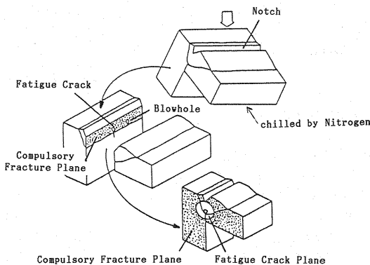
Fig.4 Observation of Fatigue Cracks
