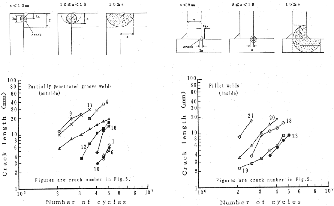
Fig.7 Changes of Fatigue Crack Size
