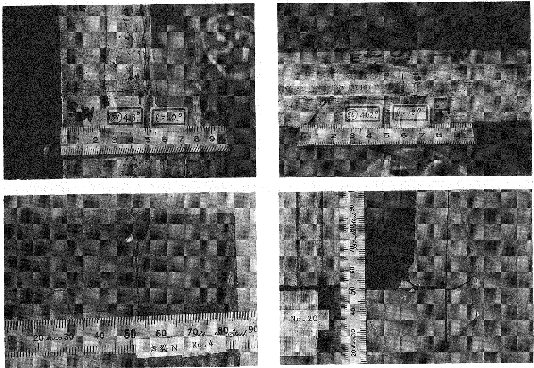
Fig.6 Fatigue Cracks
