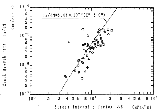
Fig.10 Fatigue Crack Propagation Rate and Stress Intensity Factor Range, obtained from Beach Marks
