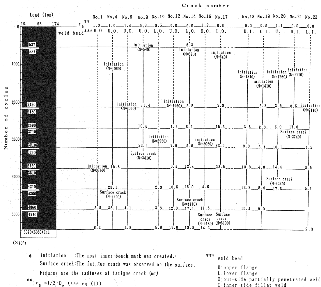
Fig.5 Load History, Initiation and Propagation of Fatigue Cracks
