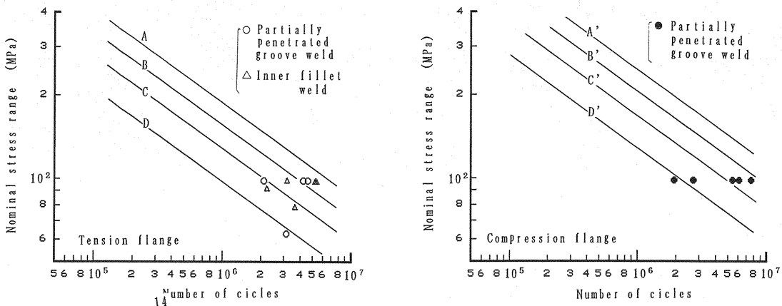
Fig.9 Fatigue Test Results (Nominal Stress Range v.s. Fatigue Life with 10mm Fatigue Crack in Diameter)
