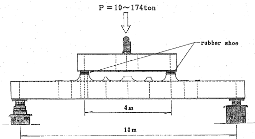
Fig.3 Test Set-up
