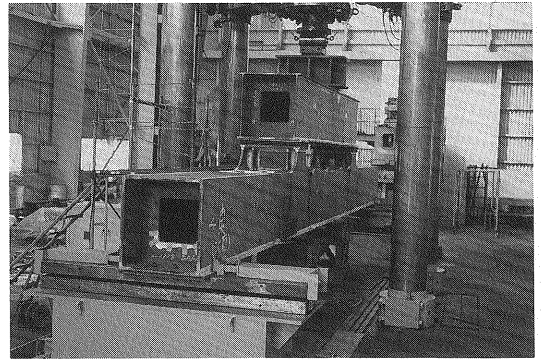
Fig.3 Test Set-up
