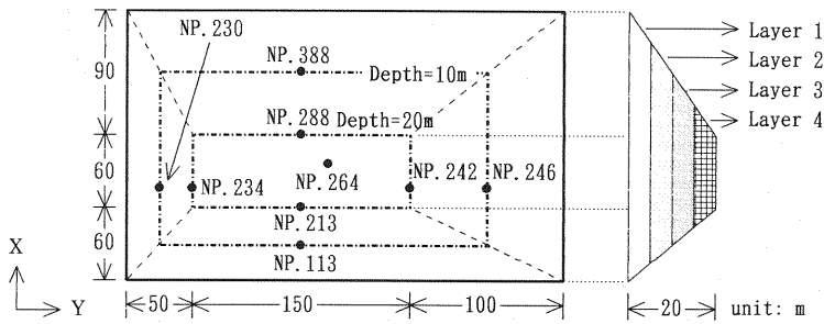
Fig.7 Configuration of the model ground to be analyzed by EXQ3D model
