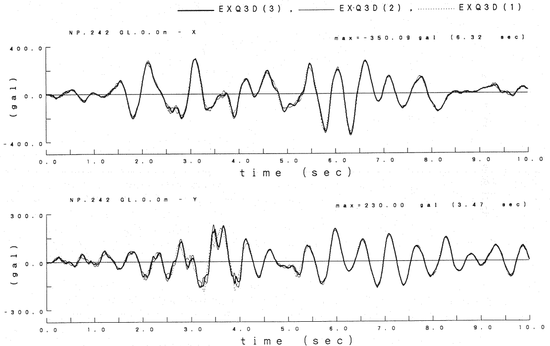
Fig.8 Influence of modal orders considered in the analyses on acceleration response (EXQ3D model)
