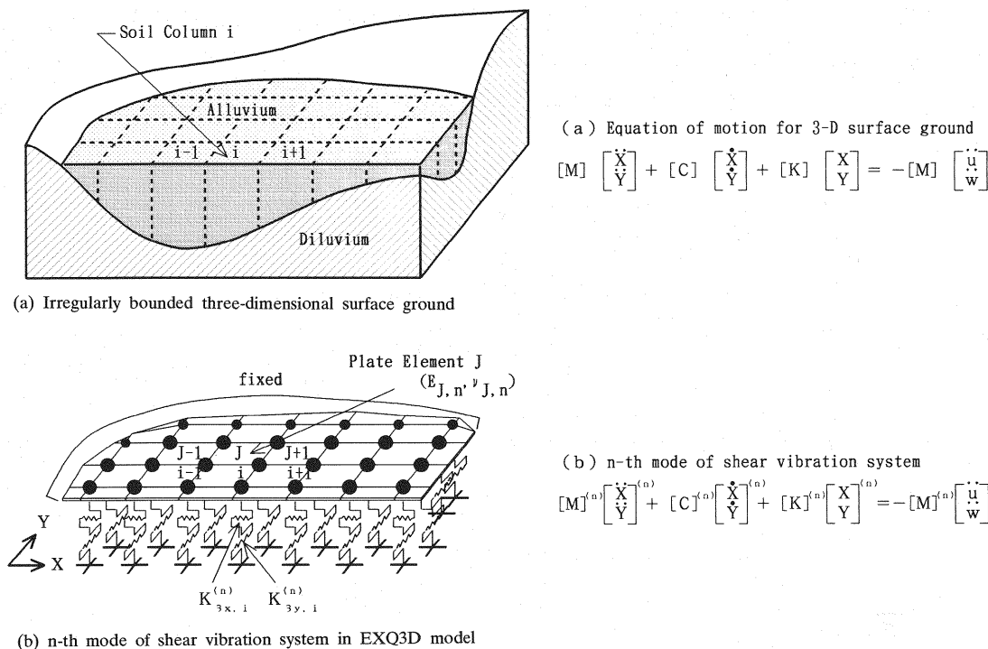
Fig.6 A schematic diagram to represent the extended quasi-three-dimensional ground model
