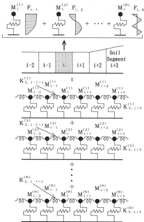
Fig.1 A schematic diagram of the extended quasi-two-dimensional ground model
