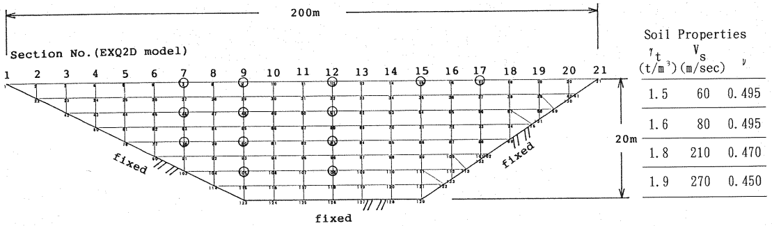
Fig.2 Two-dimensional model ground used in the analyses by EXQ2D and FEM2
