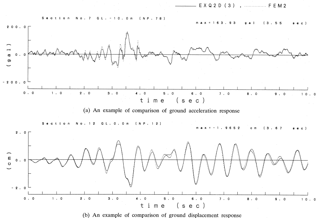
Fig.5 Examples of the comparison of the results between EXQ2D model and finite element model (FEM2)
