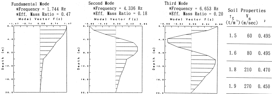
Fig.3 Fundamental through third shear vibration modes of the soil layer in the central region of the model ground
