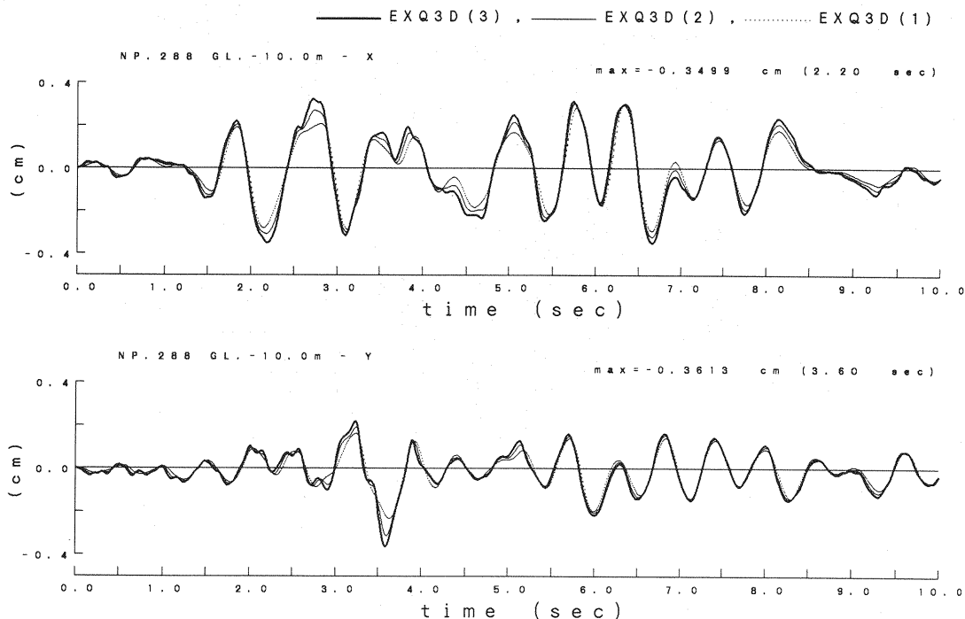
Fig.9 Influence of modal orders considered in the analyses on displacement response (EXQ3D model)
