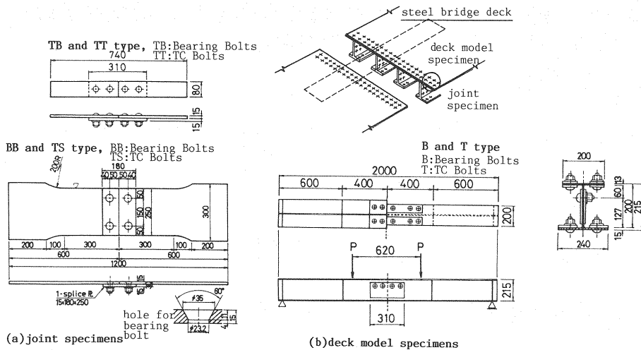
Fig.1 Configurations and Dimensions of Specimens.
