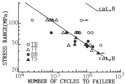
Fig.2 Fatigue Test Results of Joint Specimens.
