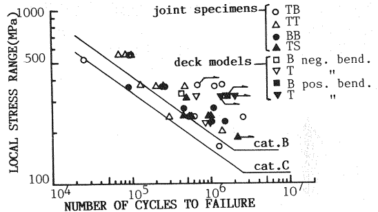
Fig. 6 Local Stress Based S-N Diagram.
