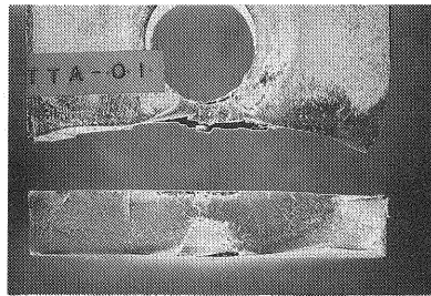
Photo 1 Failure Surface of TT-type Joint Specimen.
