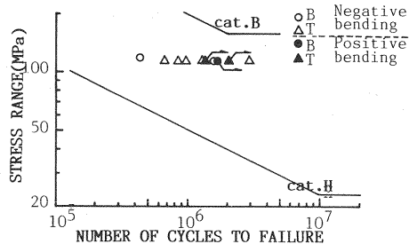
Fig.3 Fatigue Test Results of Deck Model Specimens.
