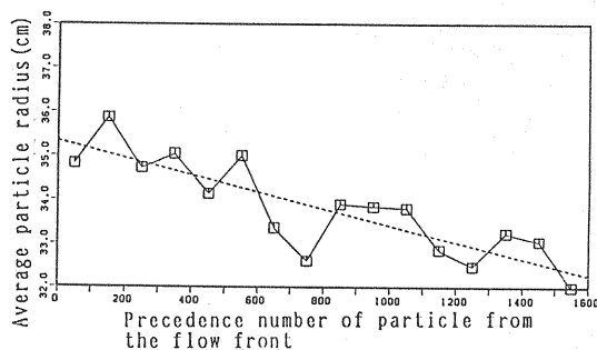
Fig.29 Particle radii distribution 19.5 sec in debris flow.
