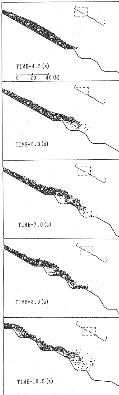
Fig.4 (a) Close-up of the debris flow with the water effect.
