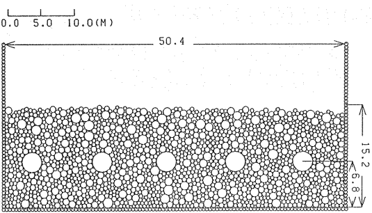
Fig.2 Granular assembly model after compaction.
