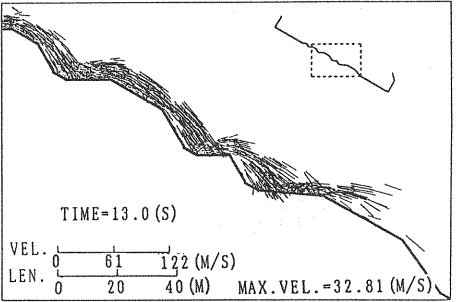
Fig.9 Velocity distribution 13.0 sec after sliding of debris flow with water effect.
