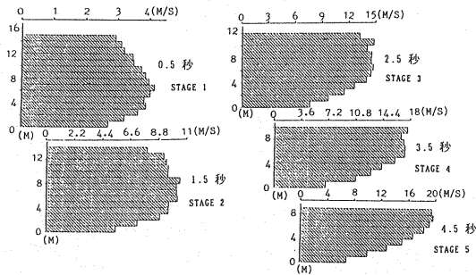
Fig.5 Flow velocity at various depths for debris flow with the water effect.
