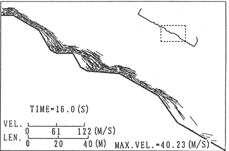
Fig.10 Velocity distribution 16.0 sec of the debris flow with the water effect.
