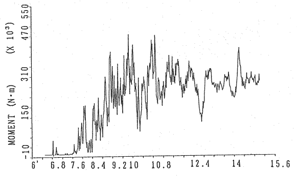
Fig.18 Total impulsive moment on a wall base caused by a debris flow.
