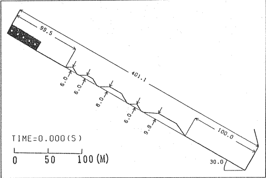
Fig.3 Rough slope [Unit: Length (m) · Angle (Degree)]
