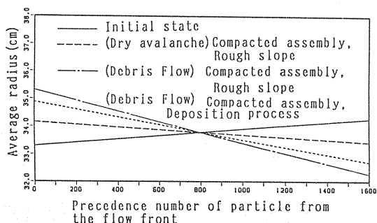
Fig.31 Particle radii distribution in cases of rock avalanche, debris flow.
