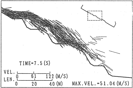
Fig.8 Velocity distribution 7.5 sec after the sliding of the compacted dry assembly.
