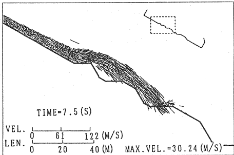
Fig.7 Velocity distribution 7.5 sec after the sliding of the debris flow with the water effect.
