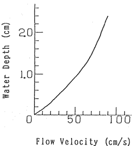
Fig.23 Theoretical velocity distribution of a debris flow.
