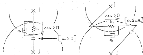
Normal direction Transverse direction Fig.1 Mechanical model at contact point.
