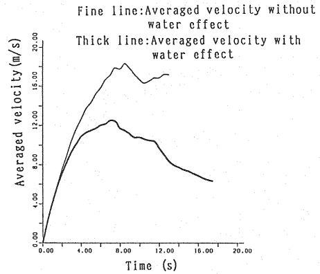
Fig.12 Average flow velocities for a dry avalanche and debris flow with water effect.
