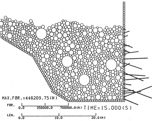
Fig.16 Impulsive force vectors on a wall due to a debris flow.
