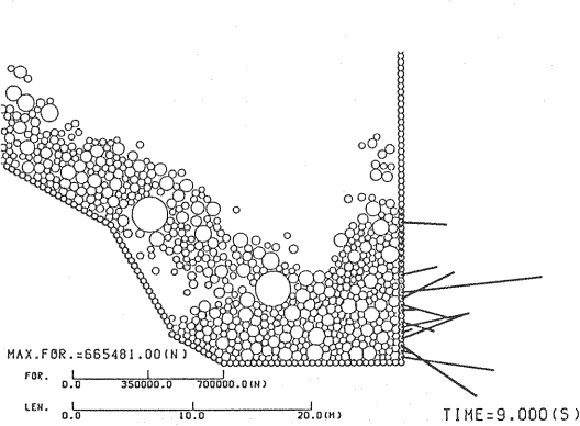
Fig.15 Impulsive force vectors on a wall due to a debris flow.
