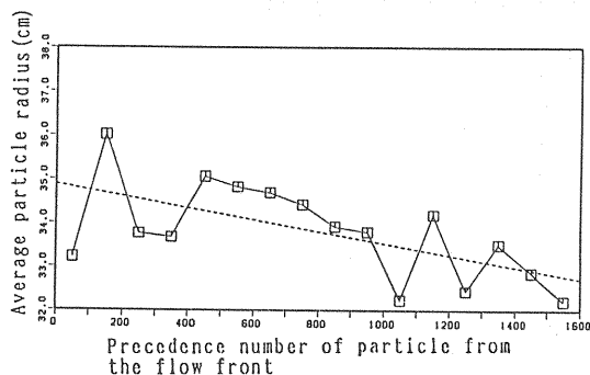
Fig.30 Particle radii distribution in deposition process at 18 sec.
