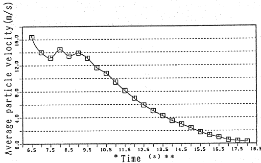
Fig.24 Averaged particle velocity versus Time.
