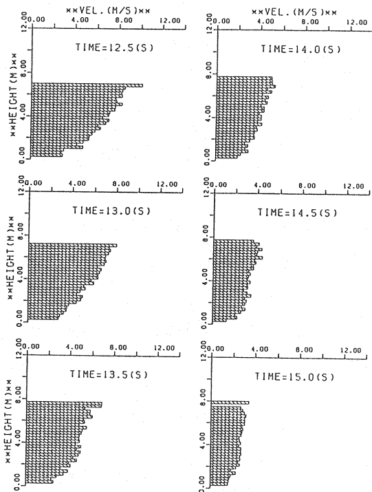
Fig.22 Velocity distribution at various heights from the bottom.
