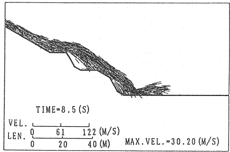
Fig.20 Particle velocity at 8.5 sec during sedimentation in a debris flow.
