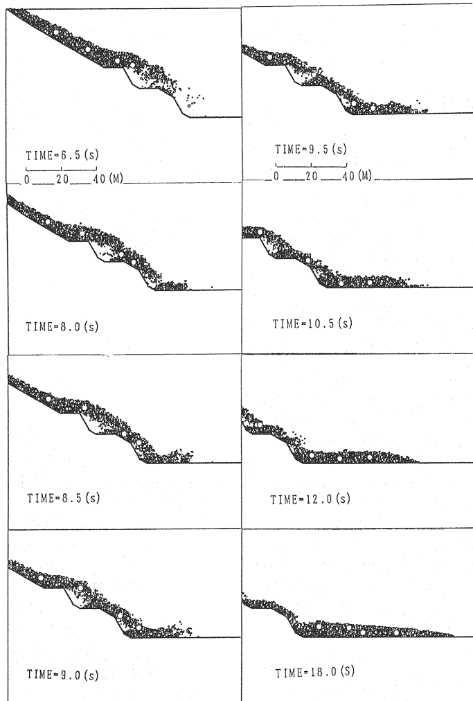
Fig.19 Deposition on process of the debris flow.
