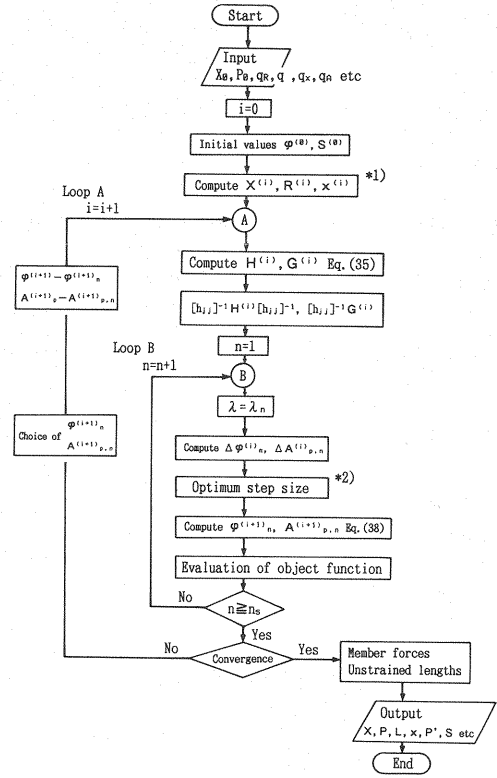
Fig.2 Flow of computation.
