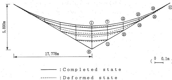
Fig.6 Completed shape and deformation.
