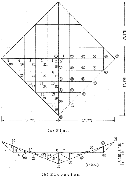
Fig.5 Example 2 : Diagonal cable net.
