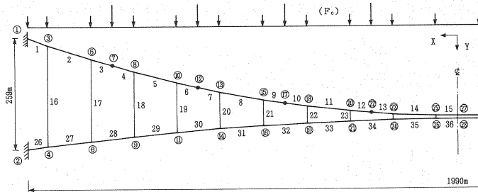
Fig.3 Example 1 : Cable girder.
