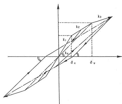
Fig. 6 Degrading trilinear characteristics.
