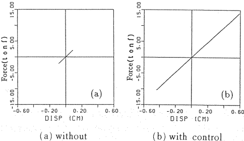
Fig.11 Force-displacement relation of the top spring.
