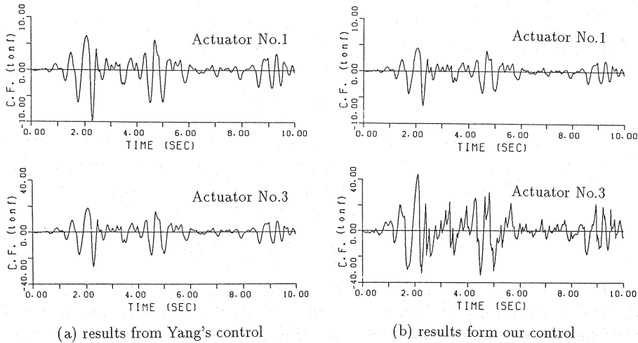
Fig.3 Control forces from the top and bottom actuators.
