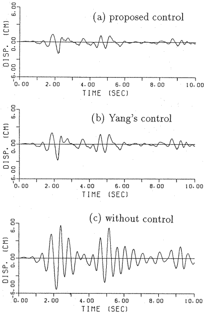
Fig.2 Relative displacement of the top floor.
