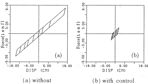
Fig.10 Hysteresis loops of the base isolator.
