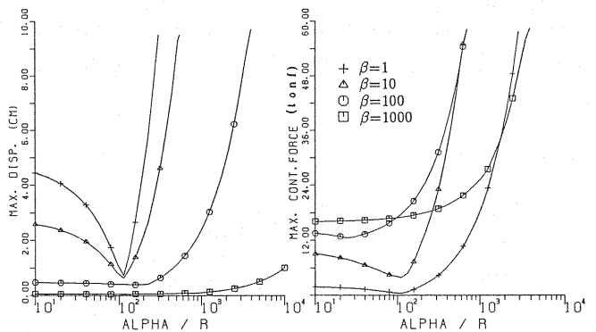
Fig. 5 Relation of \alpha/R_{11} to the maximum relative displacement of the top floor and the maximum control force of the top actuator.
