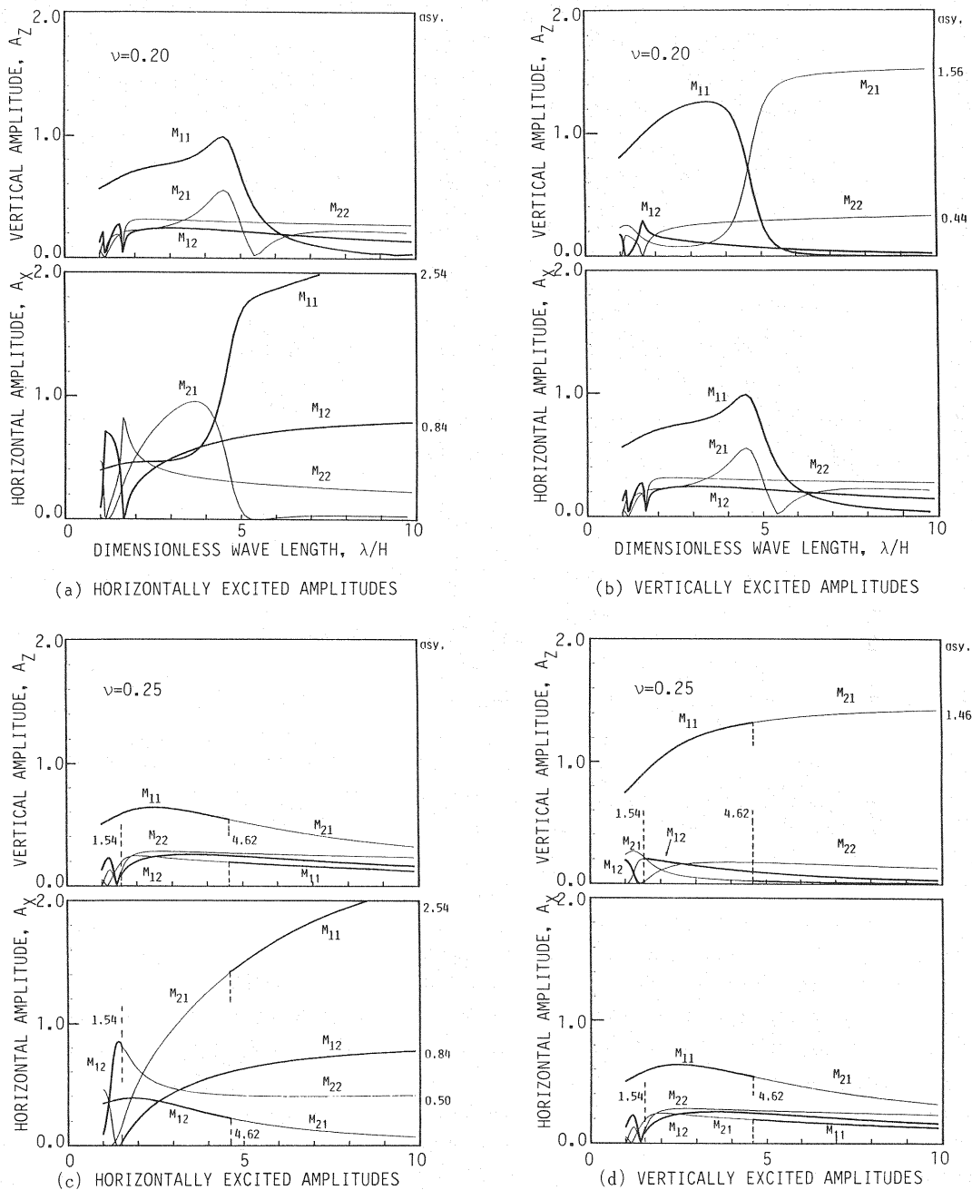
Fig.5 Amplitudes of Response to Horizontal or Vertical Excitation (Continued).
