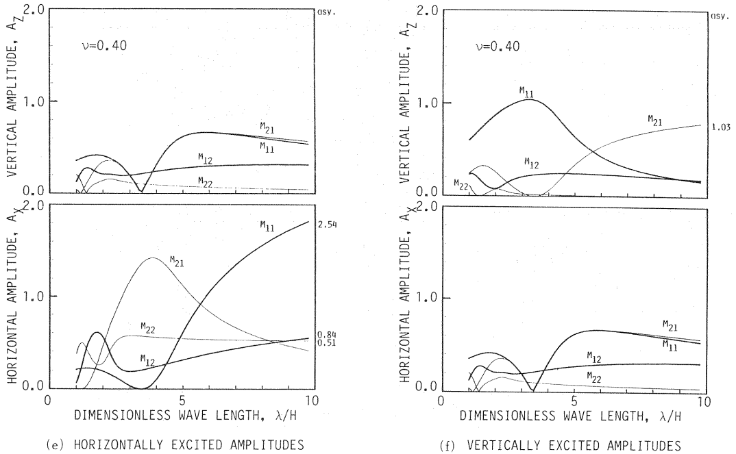
Fig.5 Amplitudes of Response due to Horizontal or Vertical Excitation.
