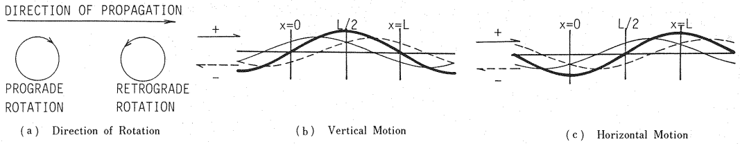
Fig. 2 Particle Motion of Stationary Vibration and Traveling Rayleigh Wave.
