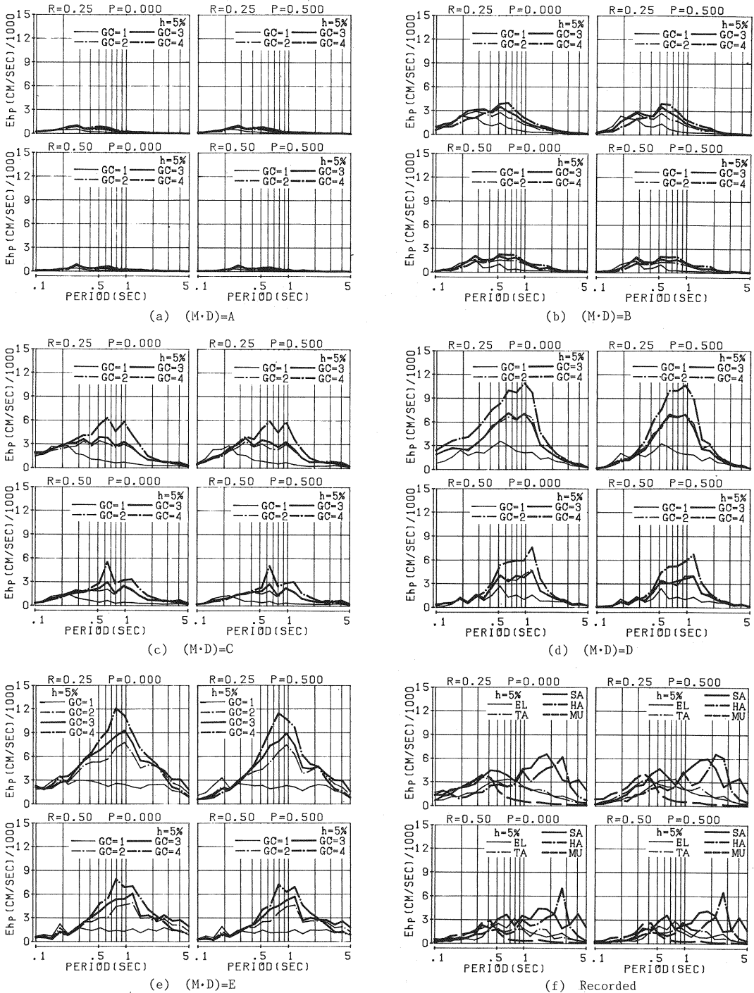
Fig. 5 Hysteretic energy response spectra.
