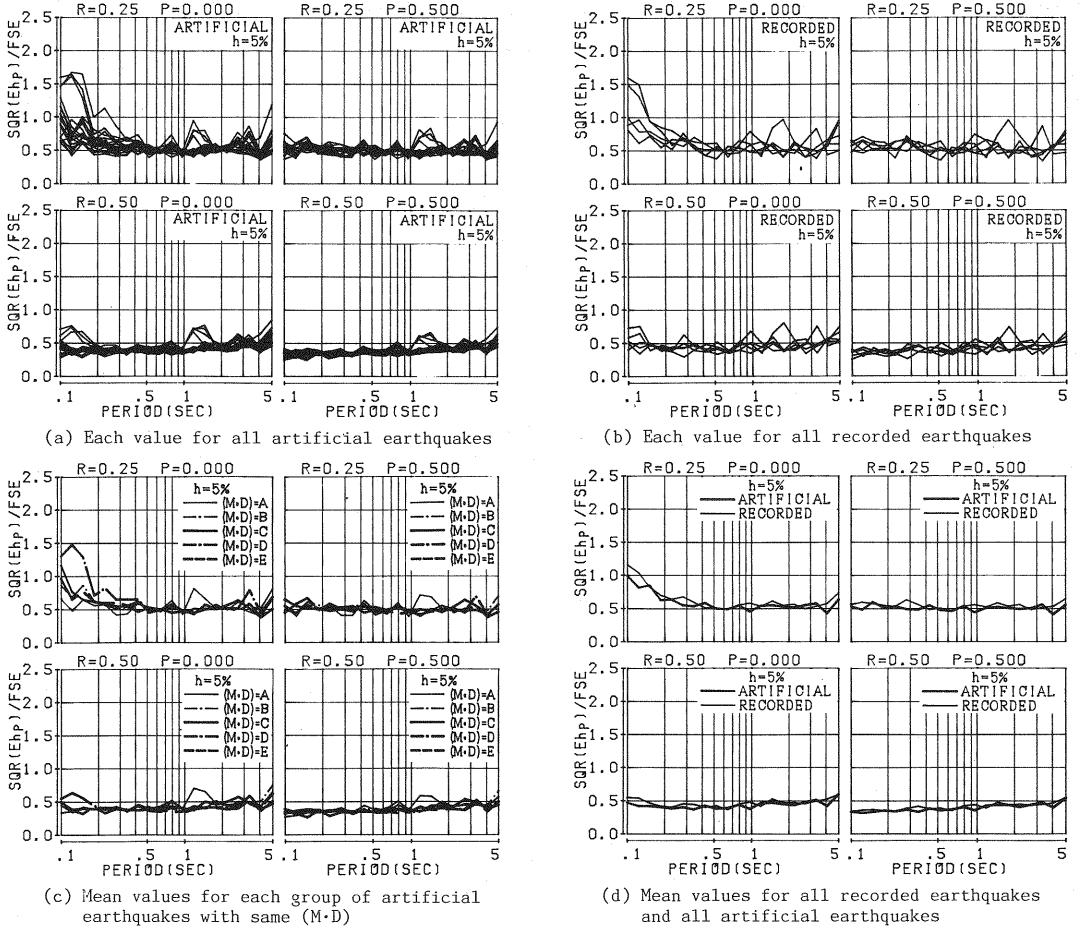
Fig. 7 Ratios of square root of hysteretic energy to effective Fourier amplitude.
