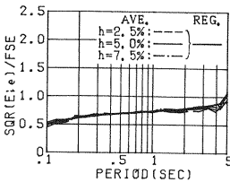
Fig. 8 Mean values and regression curve for \sqrt{E_{ie}}/F_{se} .
