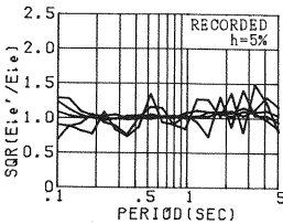
Fig. 10 \sqrt{E'_{ie}}/E_{ie} for recorded earthquakes.
