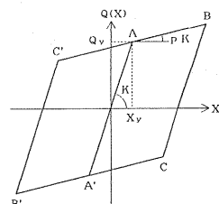
Fig. 2 Bi-linear model.
