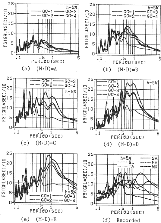
Fig.1 Fourier amplitude spectra for input earthquake motions.
