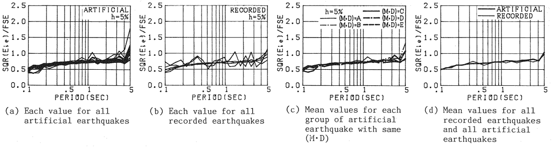
Fig. 6 Ratios of square root of elastic input energy to effective Fourier amplitude.
