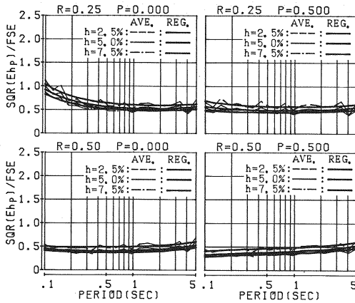
Fig.9 Mean values and regression curves for \sqrt{E_{hp}}/F_{se} .
