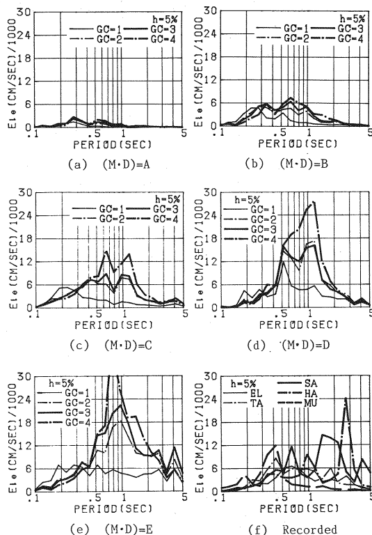
Fig. 4 Elastic input energy response spectra.
