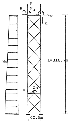
Fig. 1 Planar tower model.
