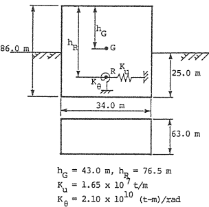
Fig. 4 Pier models of Akashi tower in plane of bridge axis.
