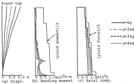
Fig. 12 Comparison of magnitude of maximum responses of planar tower model.
