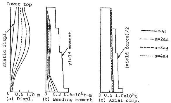
Fig. 9 Comparison of magnitude of maximum responses of planar tower-cable model.
