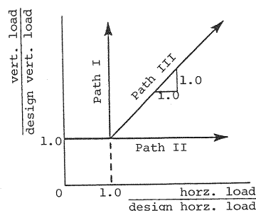
Fig.5 Loading paths.
