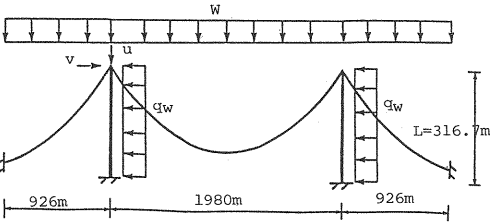
Fig. 2 Planar tower-cable model.
