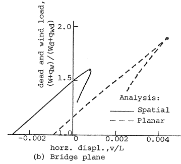
Fig. 7 Load-displacement curves due to loading path III.
