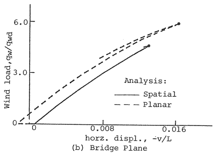
Fig. 6 Load-displacement curves due to loading path II.
