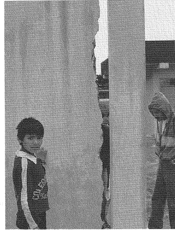
Photo 4 No Connecting Steel Bar between the Column and Wall (Equador Earthquake 1987).
