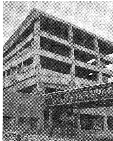
Photo2 Cracks in a Concrete Frame (Mexico Earthquake 1985).
