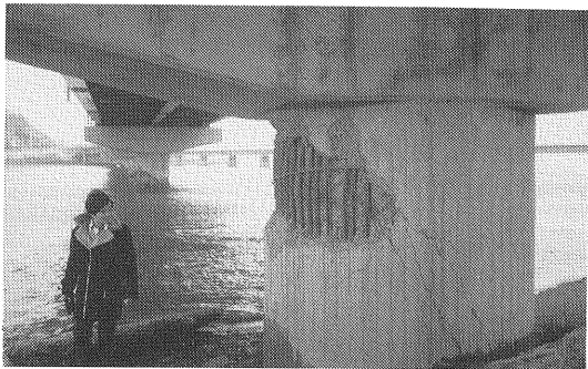
Photo6 Fracture of an RC Structure at the point of Discontinuous Reinforcement (Off-Urakawa Earthquake 1982).
