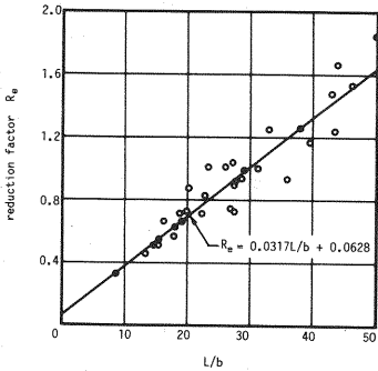
Fig.17 Reduction Factor for the Case of Eccentrically Distributed Live Load.
