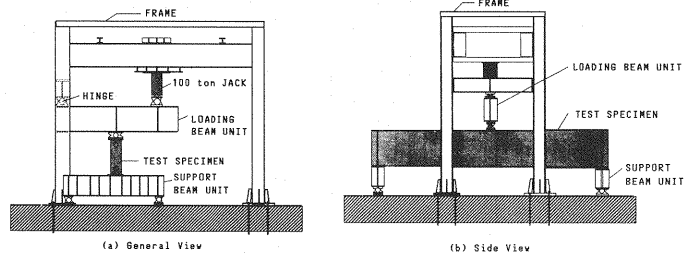
Fig. 3 Setup of a Test Beam.
