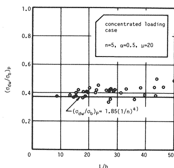
Fig. 16 Relationships between Distortional Stress and L/b for Concentrated Load.
