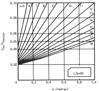
Fig. 23 Relationships between \sigma_{dw}/\sigma_{design} and Central Angle, (for L/b=50 )
