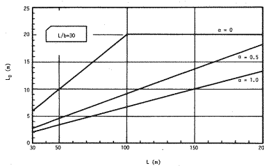
Fig. 24 Proposed Intervals of the Intermediate Diaphragms.
