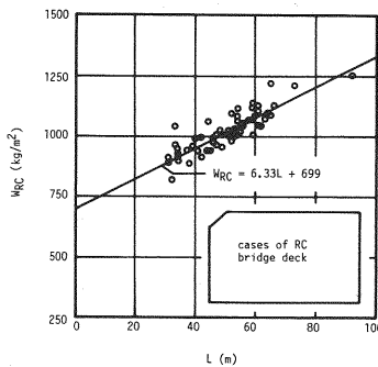
Fig. 12 Relationships between Dead Load and Span Length for Reinforced Concrete Bridge Deck.
