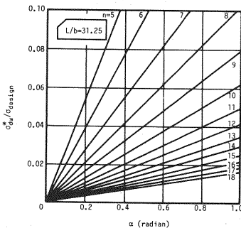
Fig.19 Relationships between \sigma_{dw}^*/\sigma_{design} and Central Angle for Eccentrically Distributed Live Load.
