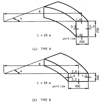
Fig. 25 Details of Box Girder for Design Examples.
