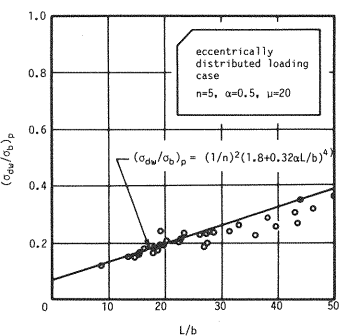
Fig. 15 Relationships between Distortional Stress and L/b for Eccentrically Distributed Load.
