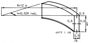
Fig. 2 Details of Tested Box Girder.
