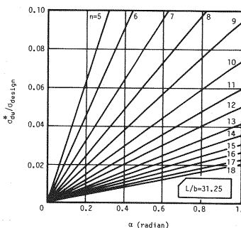
Fig.20 Relationships between \sigma_{dw}^*/\sigma_{design} and Central Angle for Uniformly Distributed Live Load.
