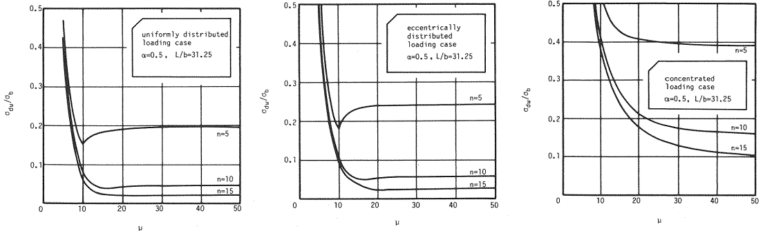
Fig. 6 Relationships between Distortional Warping Stress and Distortional Stiffness Parameter. Fig. 7 Relationships between Distortional Warping Stress and Distortional Stiffness Parameter. Fig. 8 Relationships between Distortional Warping Stress and Distortional Stiffness Parameters.
