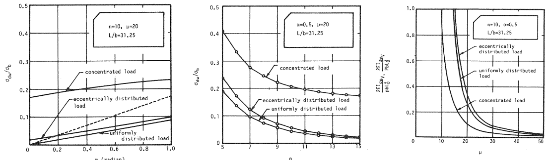
Fig. 9 Relationships between Distortional Warping Stress and Central Angle. Fig. 10 Relationships between Distortional Warping Stress and Number of the Diaphragm Intervals. Fig. 11 Relationships between Distortional Displacement and Distortional Stiffness Parameter.
