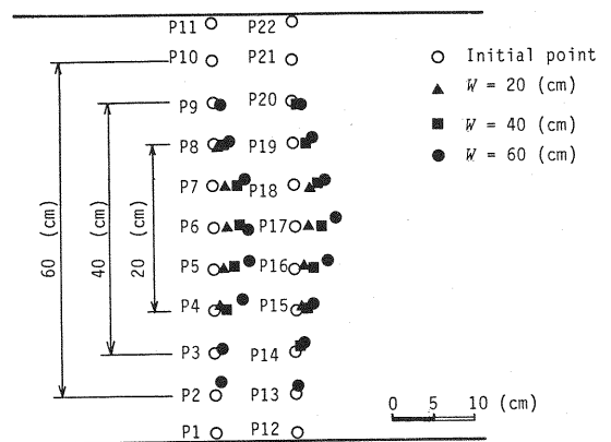
Fig. 4 Distribution of residual permanent ground displacement.
