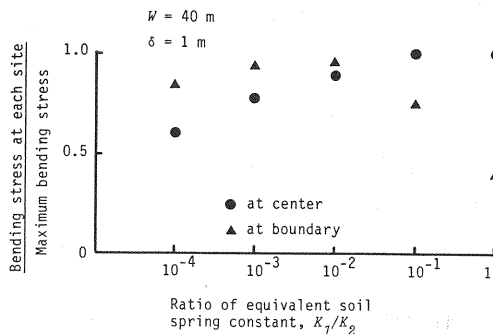
Fig. 13 Relationship between ratio of equivalent soil spring constant and ratio of bending stress to maximum bending stress.
