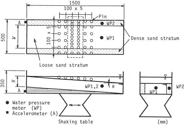
Fig.1 General view of experimental apparatus.
