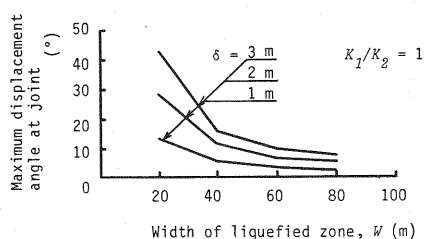
Fig. 9 Relationship between width of liquefied zone and maximum displacement angle at joint ( K_1/K_2=1 ).
