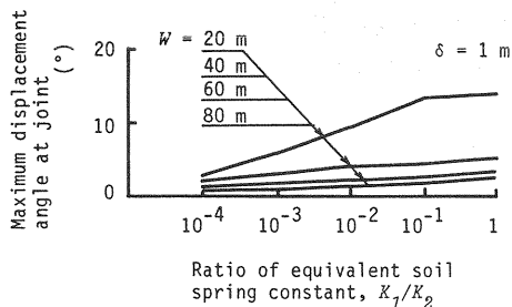
Fig. 11 Relationship between ratio of equivalent soil spring constant and maximum displacement angle at joint ( \delta=1 m).
