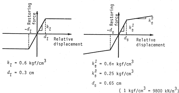
Fig. 8 Characteristic curves of equivalent soil spring constant.
