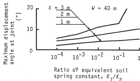
Fig. 12 Relationship between ratio of equivalent soil spring constant and maximum displacement angle at joint ( W=40 m).
