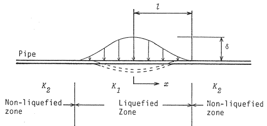
Fig.6 Analytical model (Plane figure).
