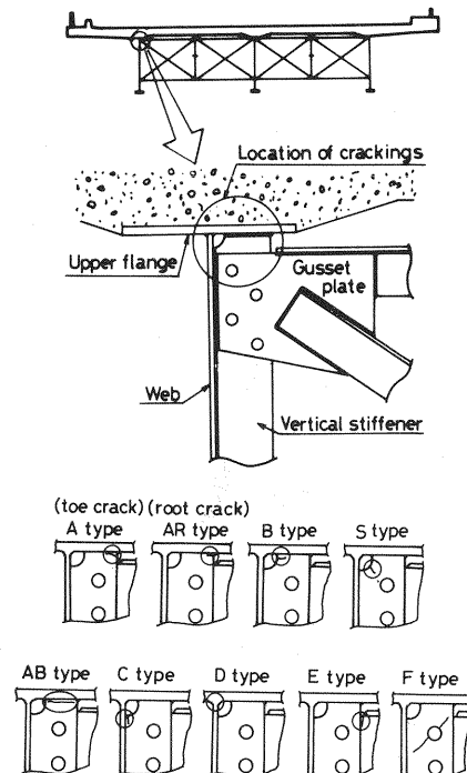
Fig.1 Types and locations of crackings.
