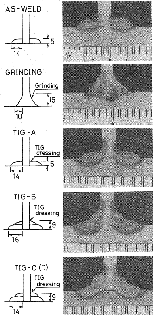
Fig. 3 Weld shapes of test specimens.
