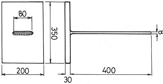
Fig. 2 Dimensions of test specimens (mm).
