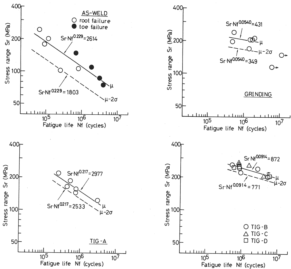
Fig.4 Results of fatigue tests.
