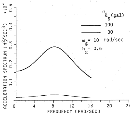
Fig. 7 Kanai's ground acceleration spectrum.
