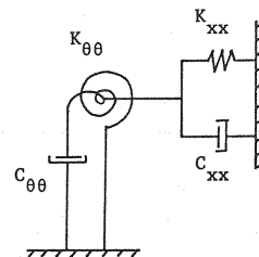
Fig.2 Modelling of pile-soil foundation.
