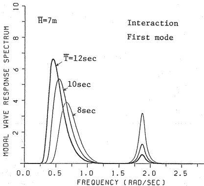
Fig.4 Modal wave response spectrum.
