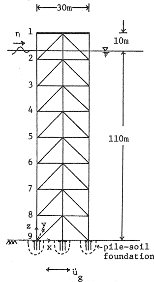
Fig.1 Analytical model of structure-pile-soil system.
