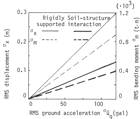
Fig. 9 RMS displacement at node 1 and RMS bending moment at node 9.
