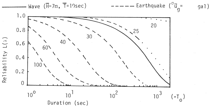
Fig. 10 Reliability of wave and earthquake loadings (Rigidly supported base).
