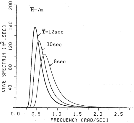
Fig.3 Bretschneider's wave energy spectrum.
