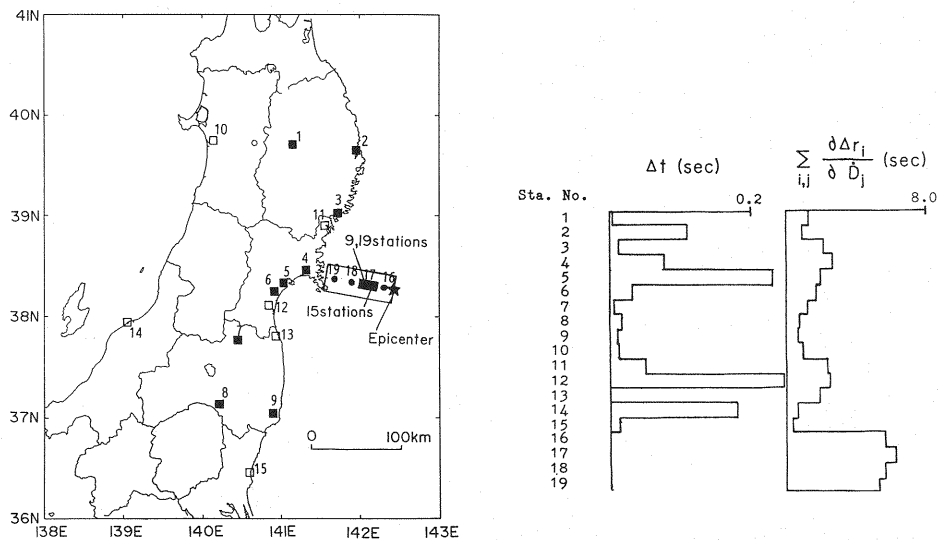
Fig. 2 Local map of the Tohoku district, showing the fault zone of the 1978 Miyagiken-oki earthquake and the locations of strong-motion recording stations. The subfault with the largest inversion uncertainty, which is determined for the case of 24 subfaults, is indicated by the shadowed portion. "Time separation", \Delta t and "moment sensitivity", \sum \frac{\partial \Delta r_i}{\partial D_j} are evaluated at individual stations for the case of 24 subfaults.
