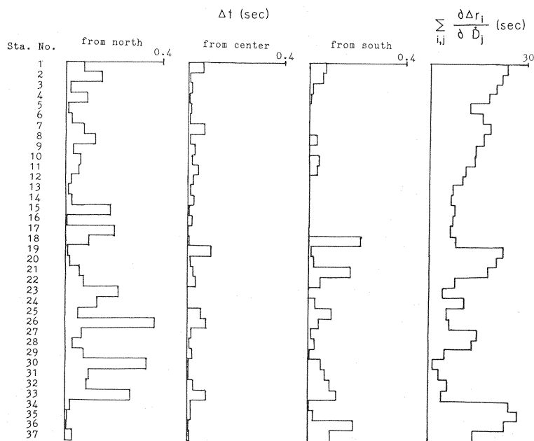
Fig.3 Local map of the Tokai district, showing the fault zone of the anticipated Tokai earthquake and the locations of strong-motion recording stations. The subfault with the largest inversion uncertainty, which is determined for the case of 40 subfaults, is indicated by the shadowed portion. "Time separation", \Delta t and "moment sensitivity", \sum_{i,j} \frac{\partial \Delta r_i}{\partial D_j} are evaluated at individual stations for three rupture modes in the case of 40 subfaults.
