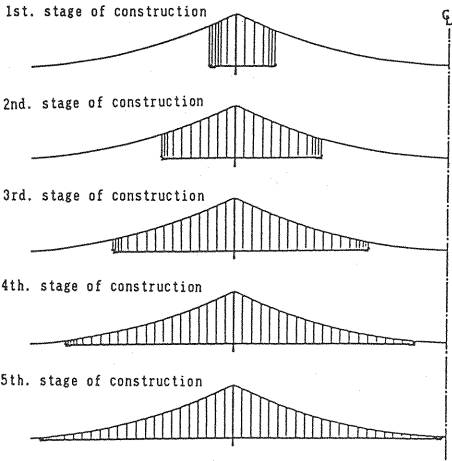
Fig. 6 Construction model of 3-spans suspension bridge.
