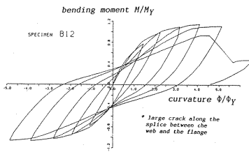
Fig.12 Moment-Curvature Relationships. B-types.
