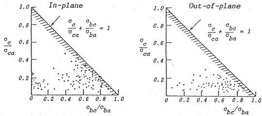
Fig.2 Interaction of the Axial Compressive Stress and the Compressive Bending Stress of Steel Bridge Piers.
