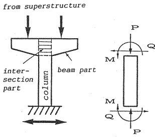
Fig.1 Modelling of T-shaped Steel Bridge Piers.
