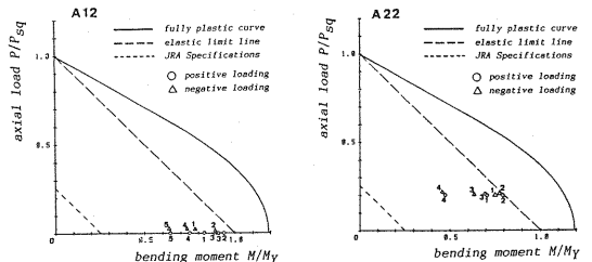
Fig.8 Interaction Curves of Axial Thrust and Bending Moment. A-types.
