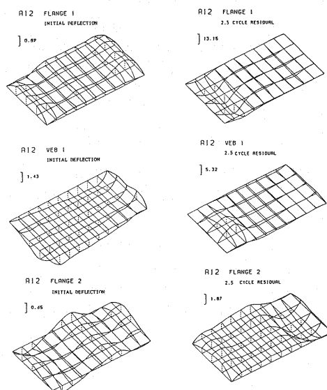
Fig. 16 Out-of-plane Deflectional Wave Forms, Specimen A 12 .
