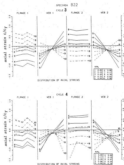
Fig. 15 Examples of Strain Distributions, Specimen B 22 .
