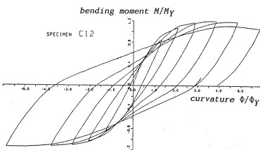
Fig.13 Moment-Curvature Relationships. C-types.
