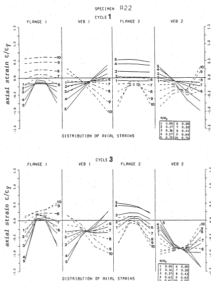
Fig. 14 Examples of Strain Distributions, Specimen A 22 .
