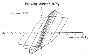
Fig.13 Moment-Curvature Relationships. C-types.
