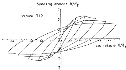
Fig.11 Moment-Curvature Relationships. A-types.
