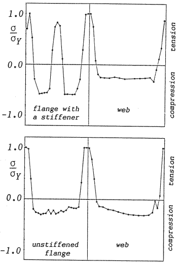
Fig.6 Measured Residual Stress Distributions.
