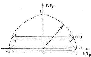
Fig. 3 Loading Types, ( i ) without Axial Thrust. ( ii ) with Axial Thrust. P/P_y=0.2 .
