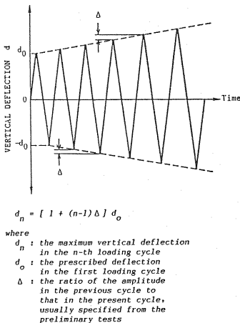
Fig.7 Sequential Ramp Wave Forms for Loading Criterion.
