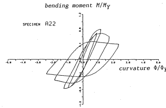
Fig.11 Moment-Curvature Relationships. A-types.
