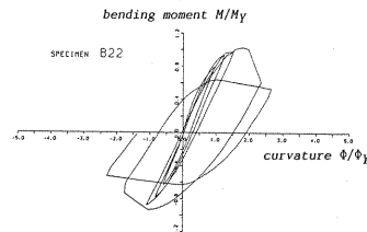
Fig.12 Moment-Curvature Relationships. B-types.
