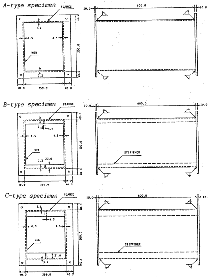
Fig. 4 Test Specimens, A, B and C.
