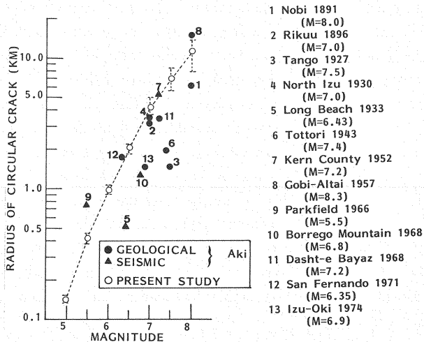
Fig.11 Comparision between Aki's results and the present ones for the crack radius-earthquake magnitude relation.
