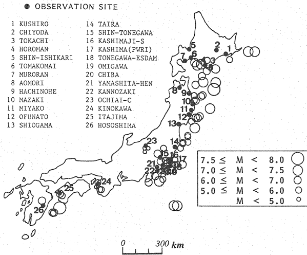
Fig.1 Map showing observation sites and earthquake origins.
