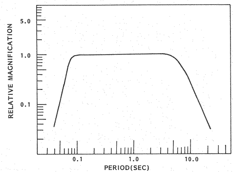
Fig.2 Overall frequency characteristics of the low pass filter and high pass filter.
