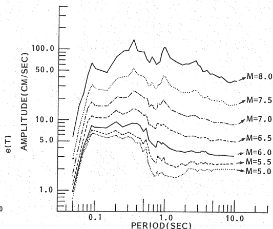
Fig. 4 Rock site spectra statistically scaled with earthquake magnitude ( \Delta=77.7 km, D=43 km).
