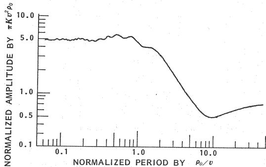
Fig.7 Expected value of far-field Fourier spectra of acceleration.
