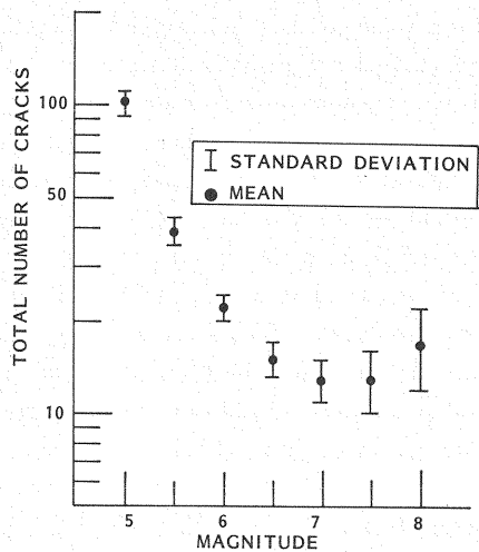
Fig.10 Relation between the total number of cracks and earthquake magnitude.
