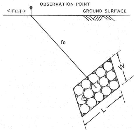
Fig.8 Schematic profile of faulting model and observation point.
