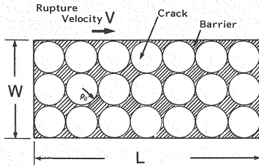
Fig. 5 Papageorgiou and Akis faulting model.
