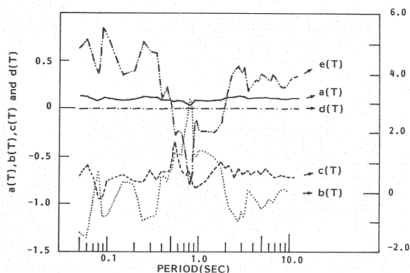
Fig. 3 Regression coefficients of the statistical analysis.
