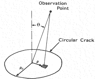
Fig. 6 Circular crack fault model.
