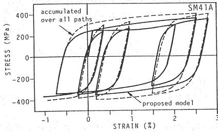
Fig. 13 Effect of estimation method of the cumulative equivalent plastic strain.
