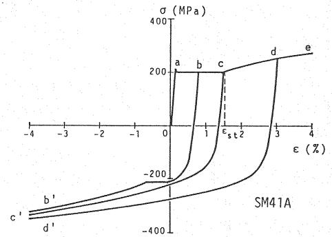
Fig. 5 Experimental stress-strain curves with unloading.
