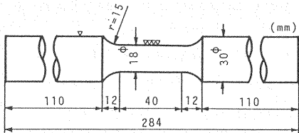
Fig. 8 Configuration of specimens.
