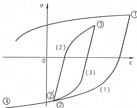
Fig. 3 Schematic figure showing ineffectiveness of a small strain amplitude on the following stress-strain relation.
