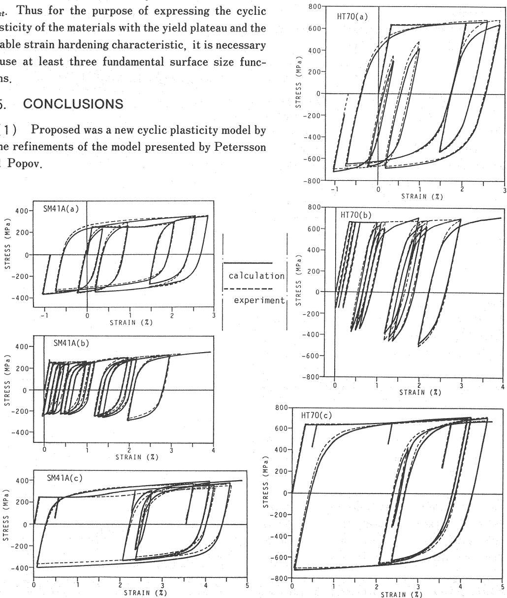
Fig. 12 Comparisons of stress-strain relations ; experiments and calculations by the proposed model.
