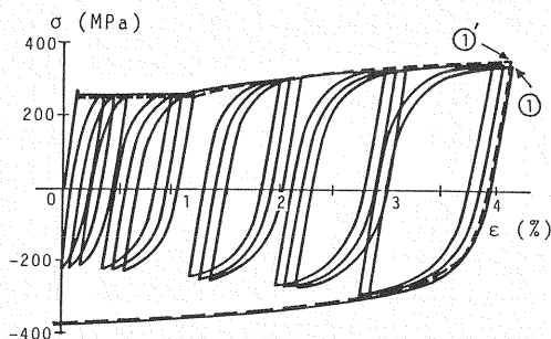
Fig. 2 Experimental stress-strain relations.
