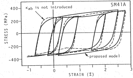
Fig. 14 Effect of the fundamental surface size function \kappa_{ab} .
