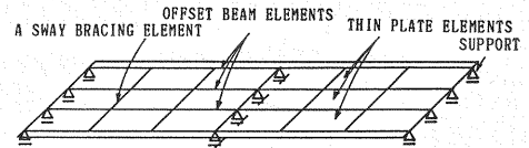
Fig. 2 Modeling of the whole structure
