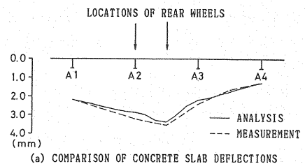
(a) COMPARISON OF CONCRETE SLAB DEFLECTIONS
