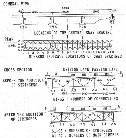
Fig.4 The three-span continuous composite girder bridge with four-main-girders to be analyzed
