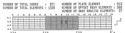
Fig.5 Element division for the analysis object
