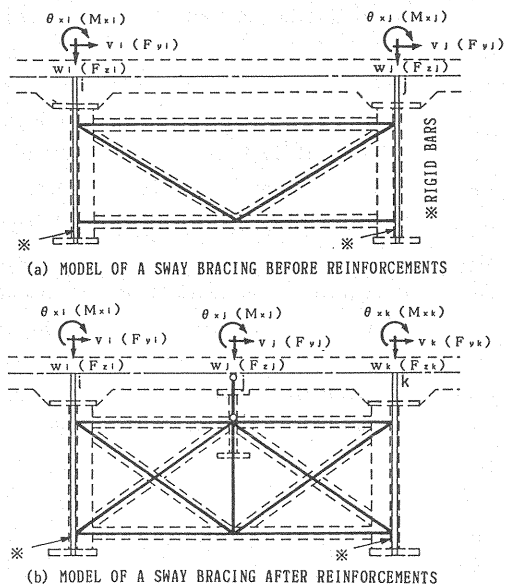
Fig.3 Modelization of sway bracings
