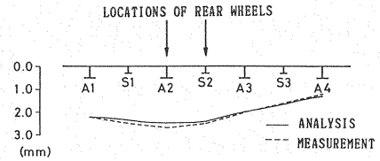
(a) COMPARISON OF CONCRETE SLAB DEFLECTIONS
