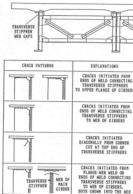
Fig. 1 Crack patterns (5)
