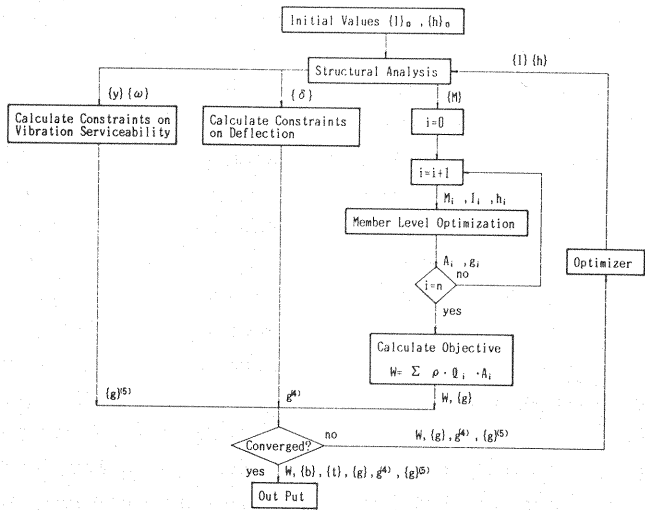
Fig. 6 Flow chart of minimum weight design of pedestrian bridge by two-level optimization.
