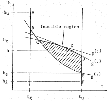
Fig. 4 Feasible region of member level optimization.
