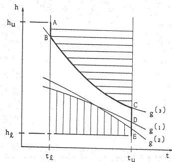
Fig. 5 The case where no feasible region exists.
