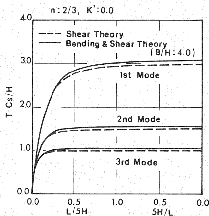
Fig. 8 Variation of non-dimensional period with L/5H or 5H/L in case of n=2/3 and K'=0.0 .
