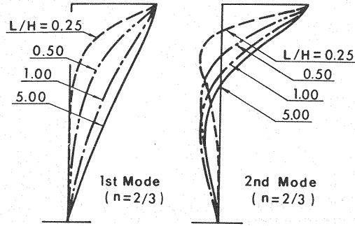
Fig. 10 The lowest two mode shapes along depth of dam by two-dimensional inhomogeneous shear beam theory.
