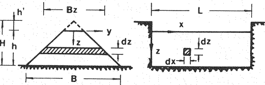
Fig.1 Two-dimensional truncated wedge modeling of dam geometry.
