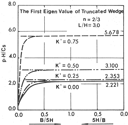
Fig. 11 Variation of non-dimensional first circular frequency of truncated wedge with B/5H or 5H/B in case of n=2/3 and L/H=3 .
