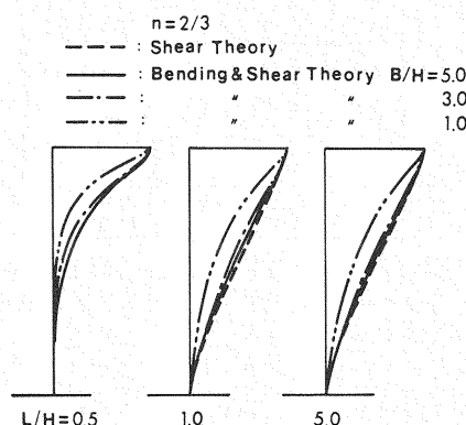
Fig. 9 Comparison of mode shapes along depth of dam between two two-dimensional beam theories.
