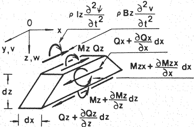
Fig.2 All forces acting on infinitesimal body.
