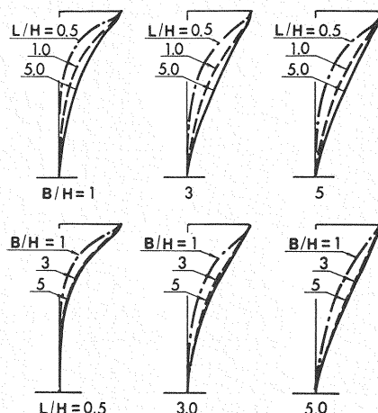
Fig. 7 Comparison of mode shapes along depth of wedge with aspects L/H and B/H in case of n=2/3 .
