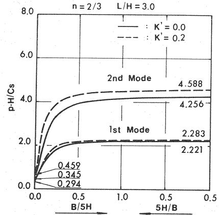
Fig. 12 Variation of non-dimensional the lowest two circular frequencies of truncated wedge with B/5H or 5H/B in case of n=2/3 and L/H=3 .
