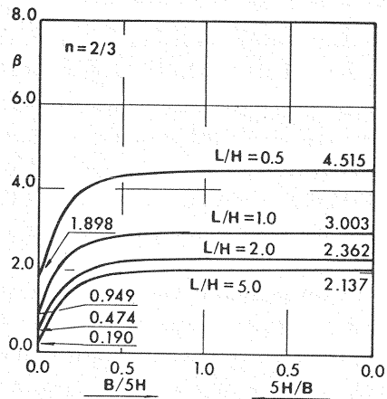
Fig. 5 Variation of the first eigen value \beta of wedge with B/5H or 5H/B in case of n=2/3 .
