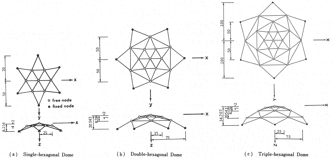
Fig. 3 Regular-Hexagonal Truss Domes.
