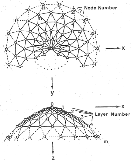
Fig. 2 General Regular-Polygonal Dome with Layers of Free Nodes.
