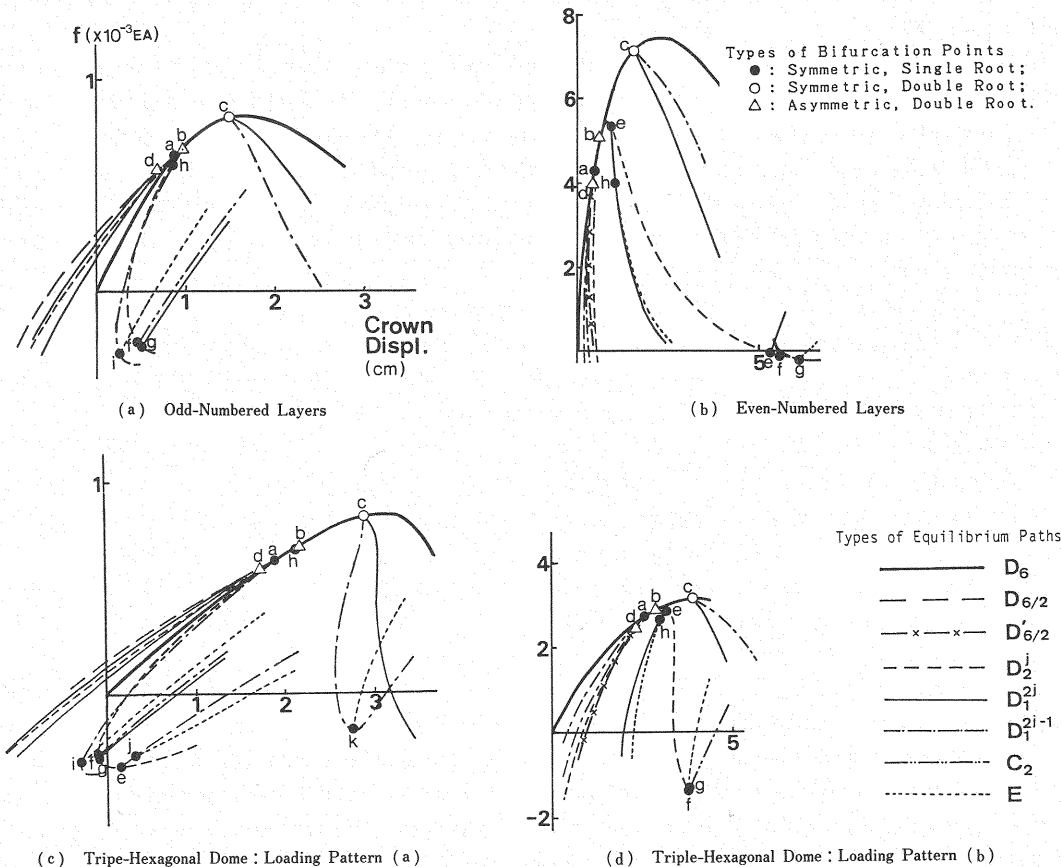
Fig. 5 Equilibrium Paths Computed for the Double and Triple-hexagonal Domes under the Loading Patterns (a) and (b).
