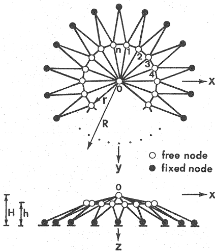
Fig. 1 Simple Regular-Polygonal Dome.
