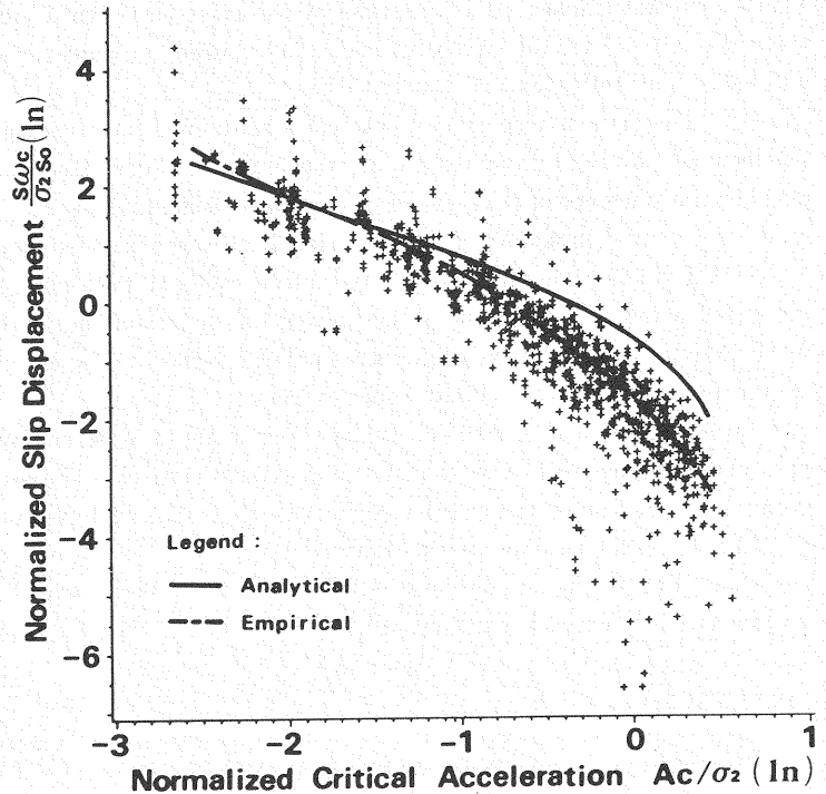
Fig. 7 Analytical Prediction and Actual Slip Displacement.
