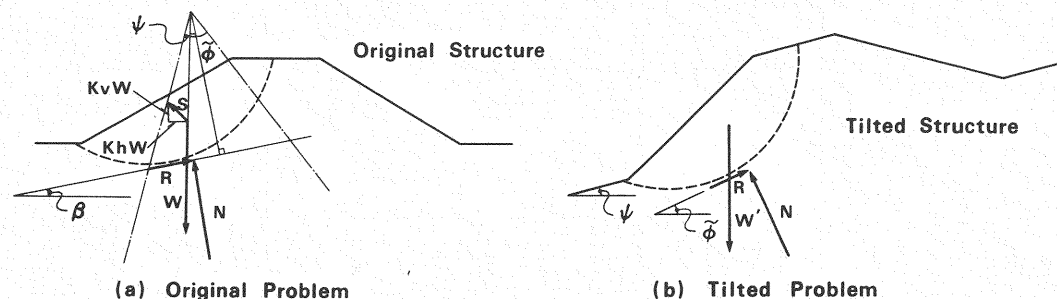
Fig.3 Pseudo-static Analysis and Equivalent Tilted Problem.
