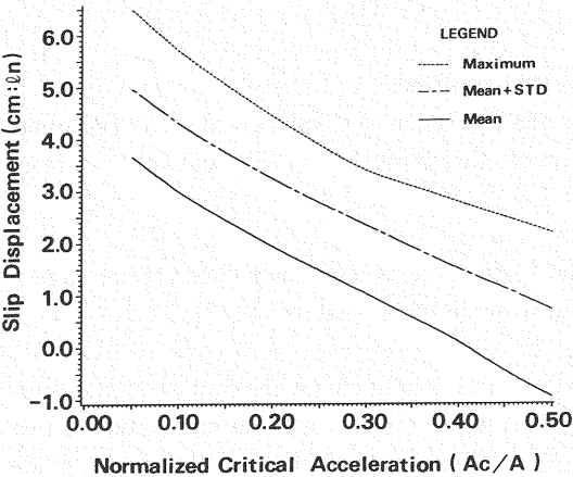
Fig.4 Slip Displacement of 52 Sets of Strong Motion Records.
