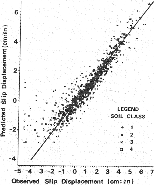
Fig.5 Predicted Slip Displacement against Observed Slip Displacement.
