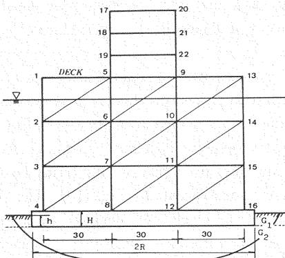
Fig. 6 Soil-Offshore Structure Model.
