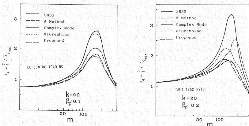
Fig. 4 Maximum Response vs Mass Ratio on the Nonproportional Damping System ( k=20 ).
