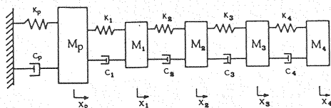
Fig. 1 Vibration Model of Nonproportional Damping Model.
