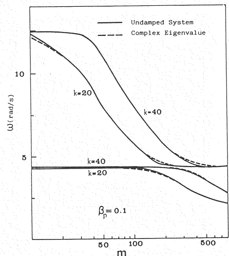
Fig. 2 Natural Frequencies vs Mass Ratio on the Nonproportional damping System.
