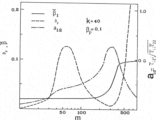
Fig. 3 Evaluations of Diagonalization and Modal Coupling Effects.
