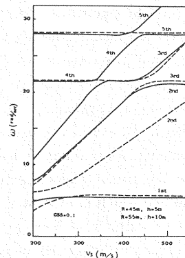
Fig. 7 Natural Frequencies vs Shear Wave Velocity on Soil-Offshore Structure Model.
