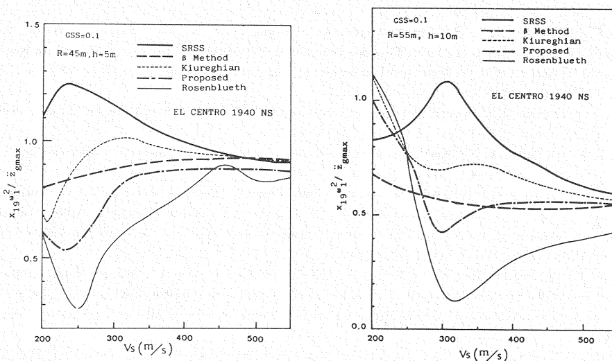
Fig. 8 Maximum Response vs Shear Wave Velocity on A Soil-Offshore Structure Model.
