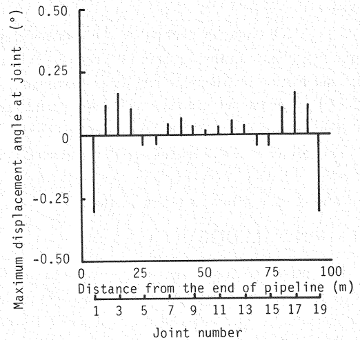
Fig. 9 Distribution of maximum displacement angle at joint (Model ground II).
