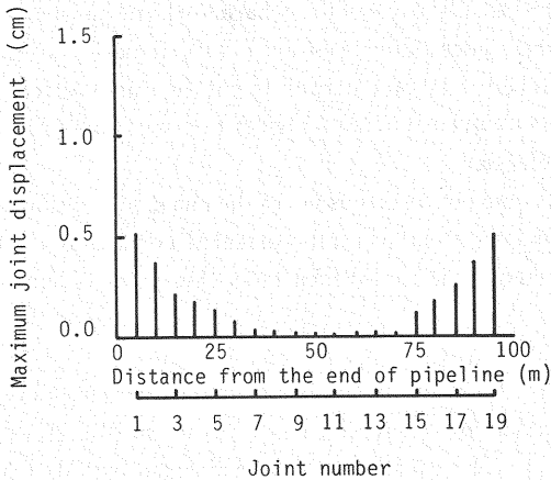
Fig. 8 Distribution of maximum joint displacement (Model ground II).
