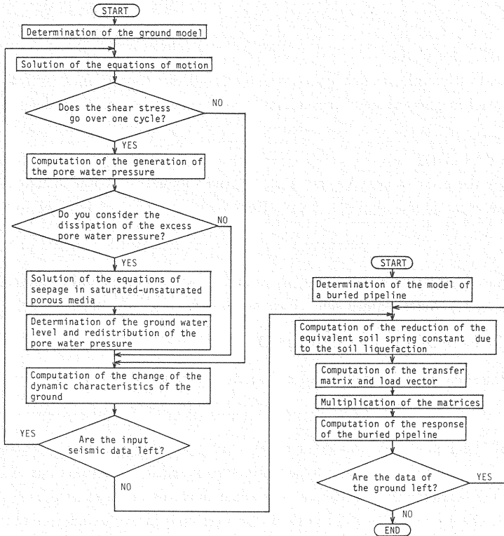
Fig.1 Simulation flow chart.
