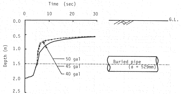
Fig. 7 Rise of the ground water level and location of the buried pipe (Model ground II).
