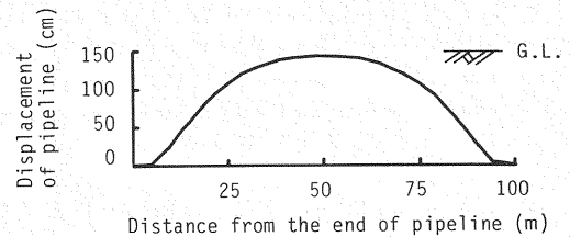
Fig. 10 Displacement of a pipeline.
