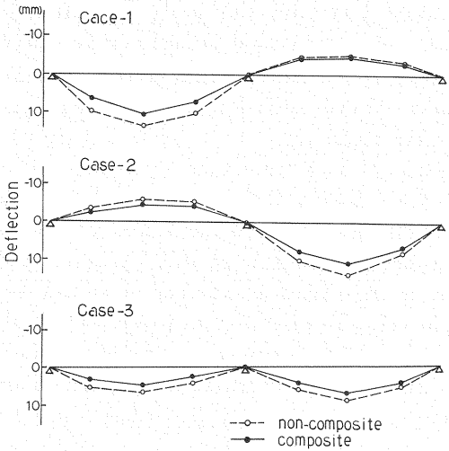
Fig. 7 Measured Deflection Curves.
