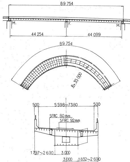
Fig. 5 Tested Bridge with SFRC Pavement.
