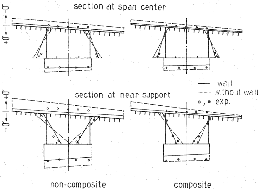
Fig. 8 Stress Distribution in Main Girder.
