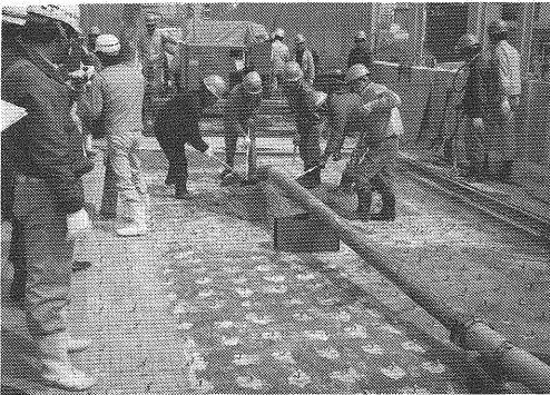
Photo 2 Casting of SFRC.
