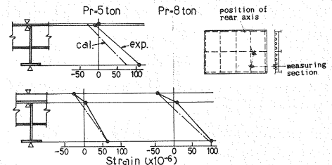
Fig. 3 Strain Distributions in Transverse Rib.
