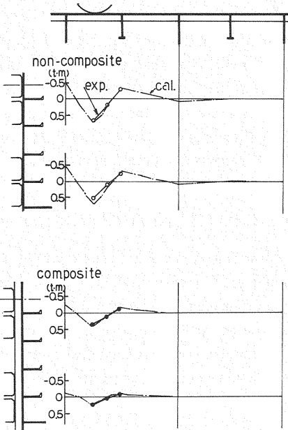
Fig. 12 Bending Moment Diagram in Longitudinal Ribs.
