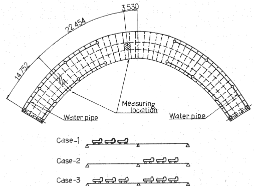
Fig. 6 Loading Cases and Measuring Locations.
