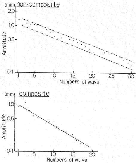
Fig. 9 Relationship between Amplitude and Numbers of Wave.
