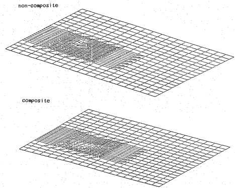
Fig. 15 Analytical Result on Deformation of Deck Structure.
