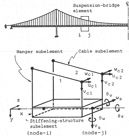
Fig. 2 Suspension-bridge element.
