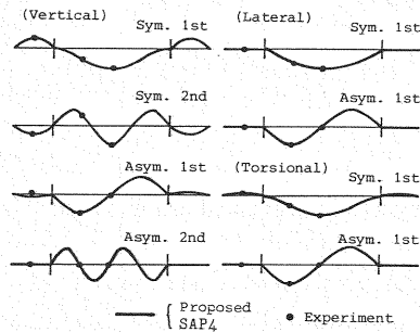
Fig.5 Natural modes of the 1/100 model of In-no-shima bridge.
