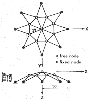
Fig. 8 8-Gonal Dome (unit in cm).
