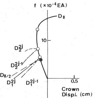
(b) Perfect Geometry
