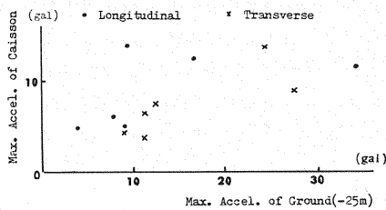
Fig.4 Maximum Accelerations of Base Ground and Caisson (P 2 ).
