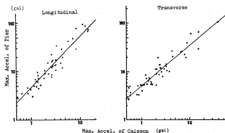
Fig.5 Maximum Acceleration of Caisson and Pier ( P_s : After the construction).
