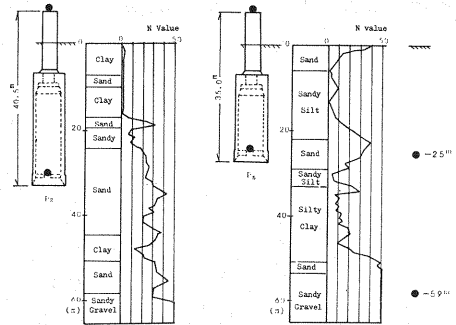
Fig.2 Caisson-Pier (P 2 , P 3 ) and Soil Profile.
