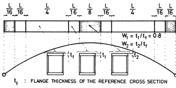
Fig. 11 Reference Thickness Change Location of Flange Plate.
