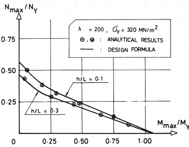
Fig. 8 Comparison of Results Predicted by the Design Formula with those Calculated by the Ultimate Strength Analysis ( \lambda=200 ).
