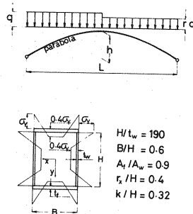
Fig.1 Arch Geometry, Loading and Reference Cross Section.
