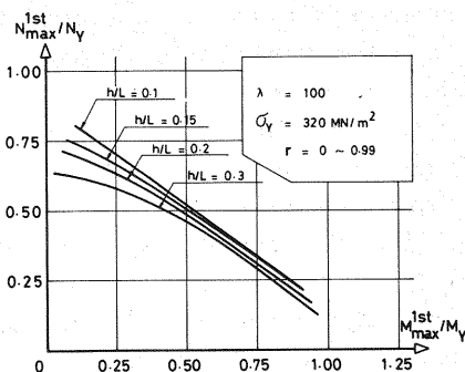
Fig. 4 Relationship Between the Maximum Force and Bending Moment (for \lambda = 100 ).
