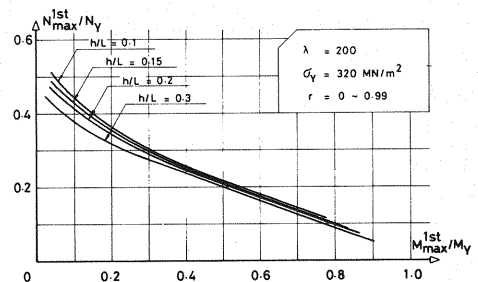
Fig. 5 Relationship Between the Maximum Force and Bending Moment (for \lambda = 200 ).
