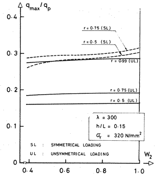
Fig. 13 Interaction Curves Between the Nondimensional Ultimate Load Intensity and Change of Flange Plate Thickness (for \lambda=300 ).
