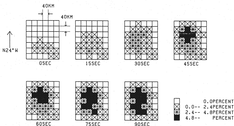
Fig. 8 The spatial distribution for the generation of short-period body-waves. The amount given at each location is an accumulation for the total process time. Symbols are the same meaning as those in Fig. 7.
