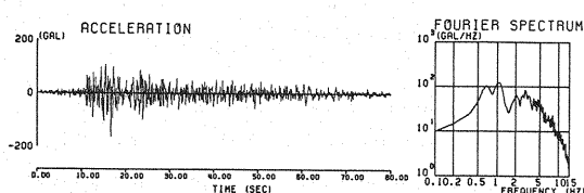
(1) Observed record
