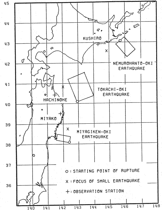
Fig. 1 The fault zones and observation stations for three earthquakes.
