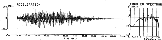
(2) Synthesized wave
