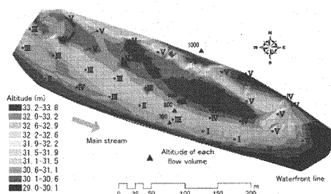
Fig. 3. Distributions of relative elevation and gravel-and-sand structure types
