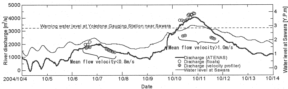
Fig. 8 Measured discharge and water level obtained by ATENAS installed at Sawara on the Tone River under torrential rain and typhoon no.22 in October 2004
