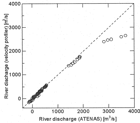
Fig. 7 Comparison of river discharge between ATENAS and the velocity profiler
